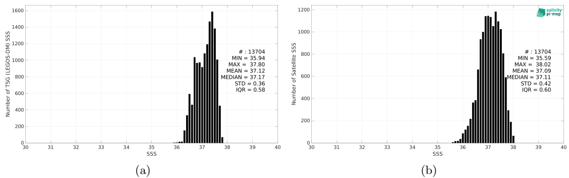
Figure 2: Histograms of SSS from TSG (LEGOS-DM) (a) and Aquarius SSS L2 OR v5 (NASA-GSFC) (b) considering all match-up pairs per bins of 0.1 over the SPURS 1 Pi-MEP region and for the full satellite product period.
