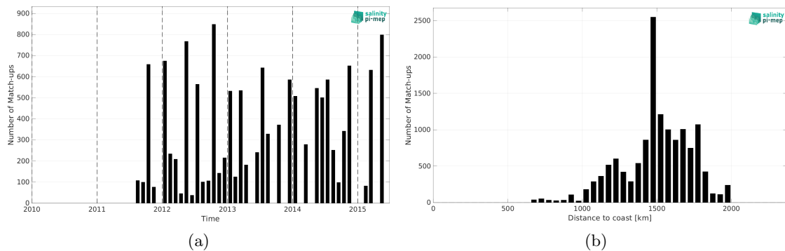
Figure 1: Number of match-ups between TSG (LEGOS-DM) and Aquarius SSS L2 OR v5 (NASA-GSFC) SSS as a function of time (a) and as function of the distance to coast (b) over the SPURS 1 Pi-MEP region and for the full satellite product period.
