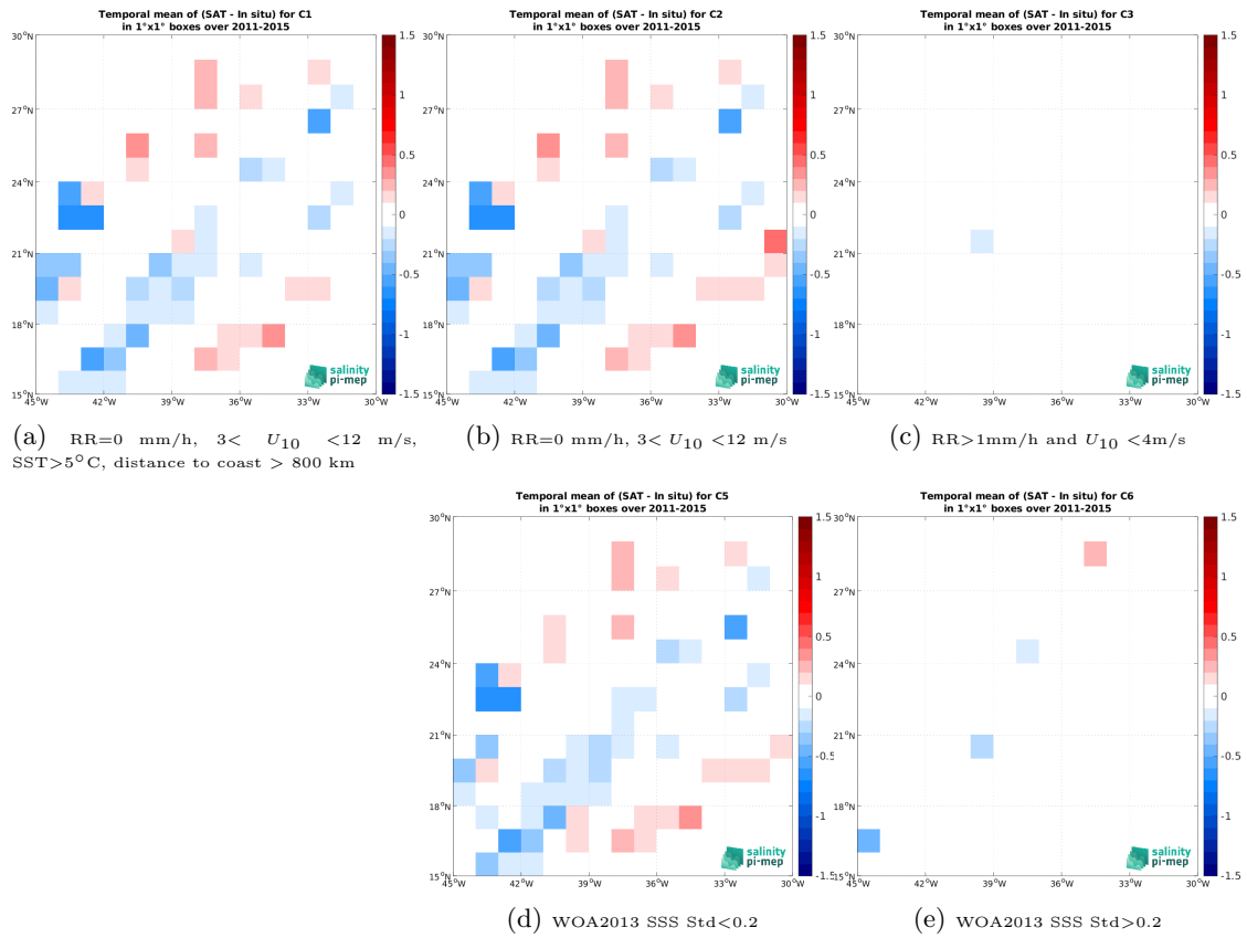
Figure 12: Temporal mean gridded over spatial boxes of size 1^\circ \times 1^\circ of \Delta\text{SSS} (Aquarius SSS L2 OR v5 (NASA-GSFC) - TSG (LEGOS-DM)) for 5 different subdatasets corresponding to:RR=0 mm/h, 3 < U_{10} < 12 m/s, SST >5^\circ\text{C} , distance to coast > 800 km (a), RR=0 mm/h, 3 < U_{10} < 12 m/s (b), RR >1 mm/h and U_{10} < 4 m/s (c), WOA2013 SSS Std <0.2 (d), WOA2013 SSS Std >0.2 (e).
