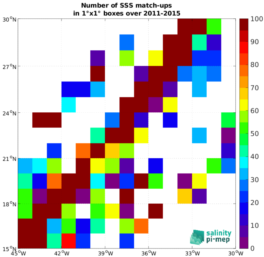
Figure 4: Number of SSS match-ups between TSG (LEGOS-DM) SSS and the Aquarius SSS L2 OR v5 (NASA-GSFC) SSS product for the SPURS 1 Pi-MEP region over 1^\circ \times 1^\circ boxes and for the full satellite product period.
