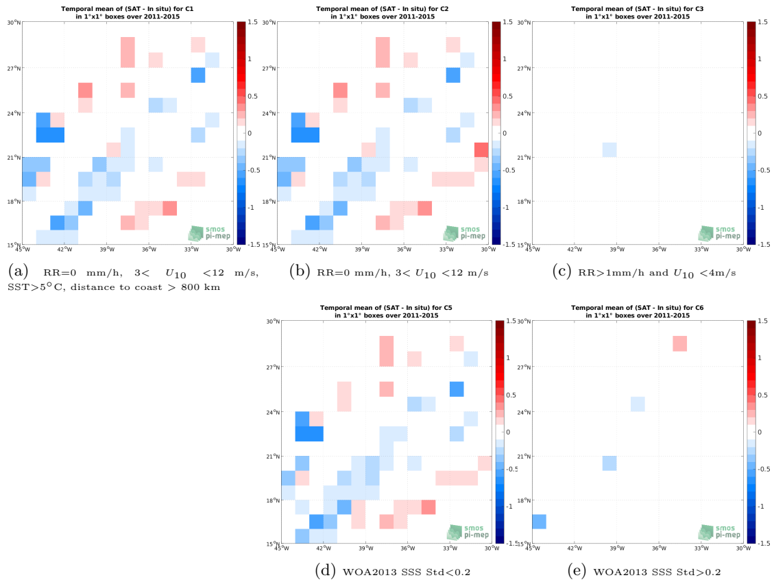
Figure 12: Temporal mean gridded over spatial boxes of size 1^\circ \times 1^\circ of \Delta SSS (Aquarius SSS L2 OR v5 (NASA-GSFC) - TSG (LEGOS-DM)) for 5 different subdatasets corresponding to: RR=0 mm/h, 3 < U_{10} < 12 m/s, SST > 5^\circ\text{C} , distance to coast > 800 km (a), RR=0 mm/h, 3 < U_{10} < 12 m/s (b), RR > 1 mm/h and U_{10} < 4 m/s (c), WOA2013 SSS Std < 0.2 (d), WOA2013 SSS Std > 0.2 (e).
