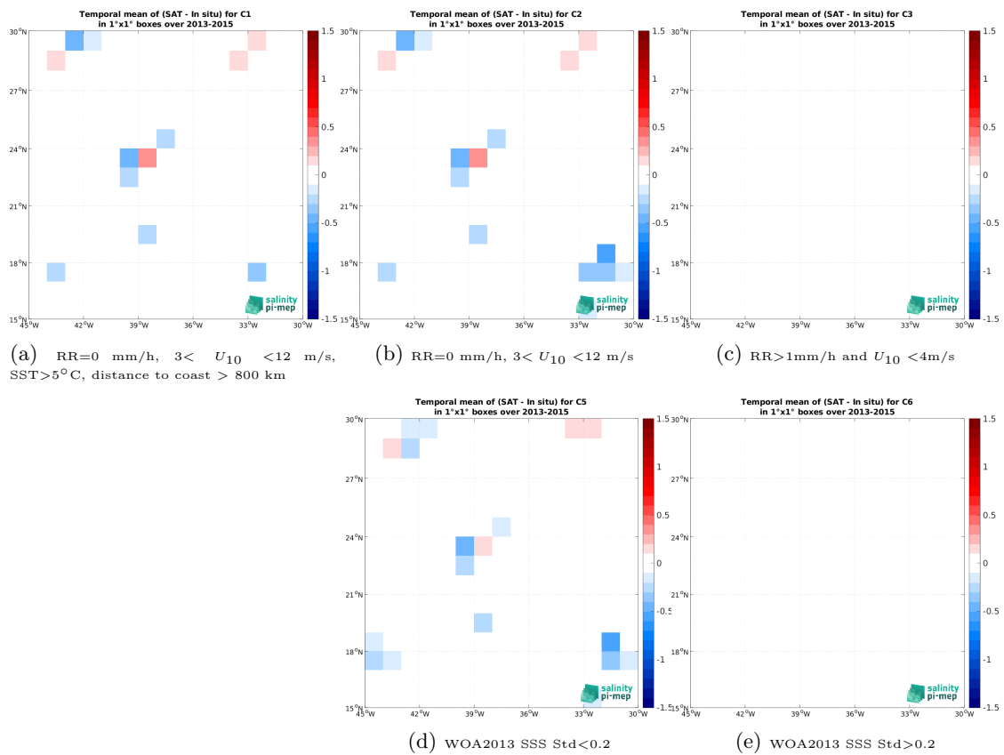
Figure 14: Temporal mean gridded over spatial boxes of size 1^\circ \times 1^\circ of \Delta SSS (Aquarius SSS L2 OR v5 (NASA-GSFC) - TSG (GOSUD-Sailing-ship)) for 5 different subdatasets corresponding to:RR=0 mm/h, 3 < U_{10} < 12 m/s, SST>5°C, distance to coast > 800 km (a), RR=0 mm/h, 3 < U_{10} < 12 m/s (b), RR>1mm/h and U_{10} < 4 m/s (c), WOA2013 SSS Std<0.2 (d), WOA2013 SSS Std>0.2 (e).
