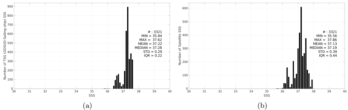
Figure 3: Histograms of SSS from TSG (GOSUD-Sailing-ship) (a) and Aquarius SSS L2 OR v5 (NASA-GSFC) (b) considering all match-up pairs per bins of 0.1 over the SPURS 1 Pi-MEP region and for the full satellite product period.
