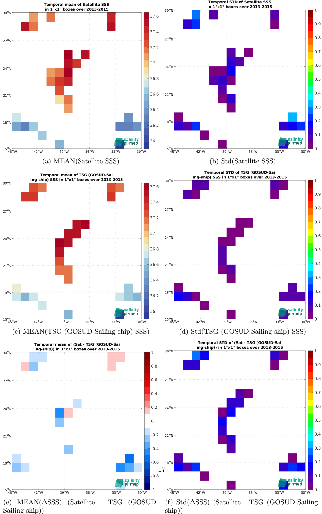
Figure 7: Temporal mean (left) and Std (right) of SSS from Aquarius SSS L2 OR v5 (NASA-GSFC) (top), TSG (GOSUD-Sailing-ship) (middle), and of \Delta SSS (Satellite - TSG (GOSUD-Sailing-ship)). Only match-up pairs are used to generate these maps.
