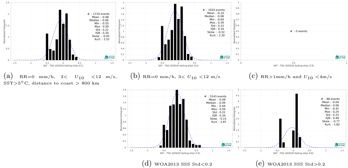
Figure 15: Normalized histogram of \Delta SSS (Aquarius SSS L2 OR v5 (NASA-GSFC) - TSG (GOSUD-Sailing-ship)) for 5 different subdatasets corresponding to: RR=0 mm/h, 3 < U_{10} < 12 m/s, SST > 5°C, distance to coast > 800 km (a), RR=0 mm/h, 3 < U_{10} < 12 m/s (b), RR > 1mm/h and U_{10} < 4 m/s (c), WOA2013 SSS Std < 0.2 (d), WOA2013 SSS Std > 0.2 (e).
