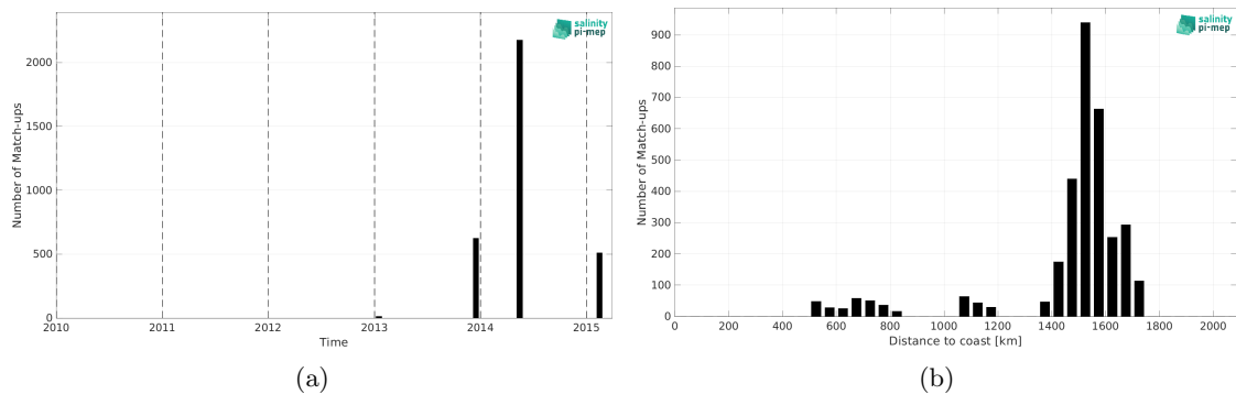
Figure 2: Number of match-ups between TSG (GOSUD-Sailing-ship) and Aquarius SSS L2 OR v5 (NASA-GSFC) SSS as a function of time (a) and as function of the distance to coast (b) over the SPURS 1 Pi-MEP region and for the full satellite product period.
