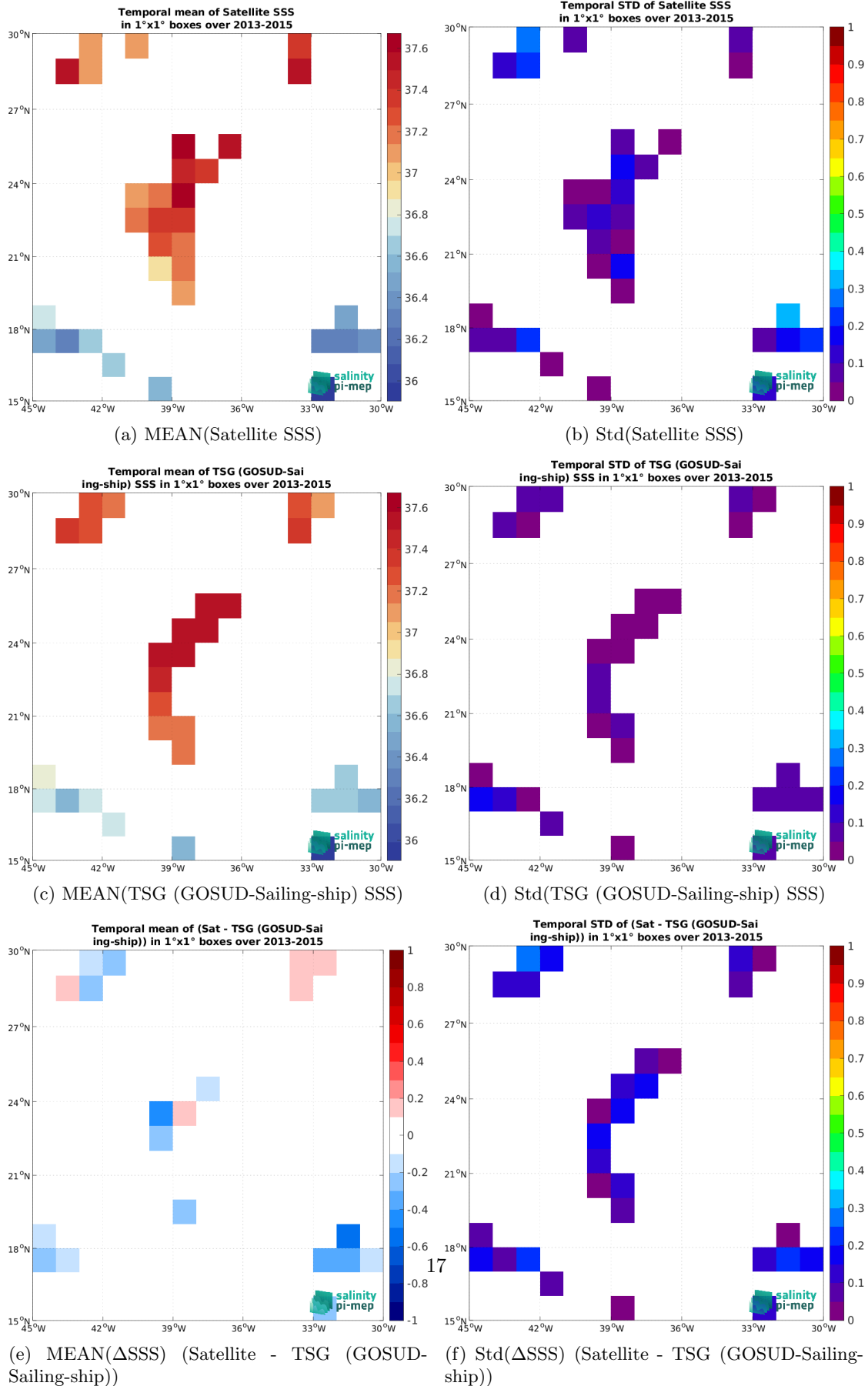
Figure 6: Temporal mean (left) and Std (right) of SSS from Aquarius SSS L2 OR v5 (NASA-GSFC) (top), TSG (GOSUD-Sailing-ship) (middle), and of \Delta SSS (Satellite - TSG (GOSUD-Sailing-ship)). Only match-up pairs are used to generate these maps.
