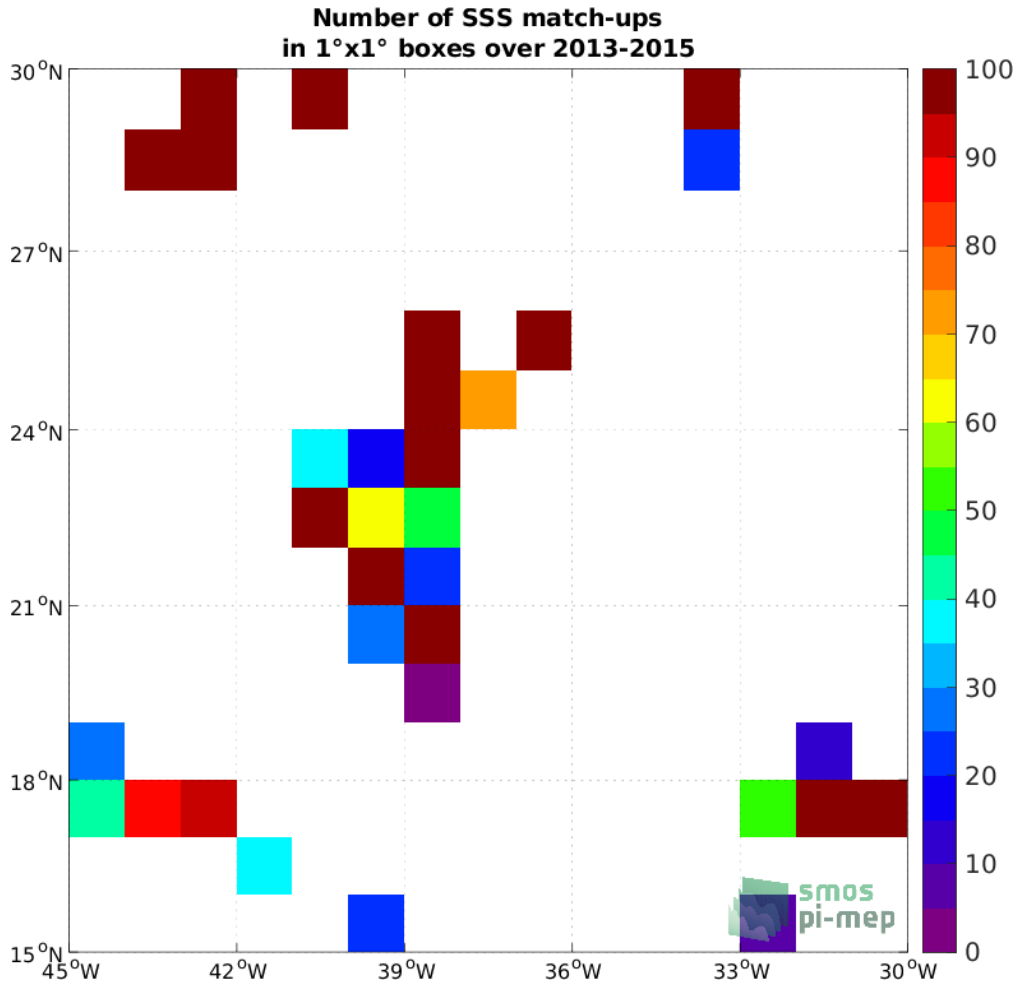
Figure 4: Number of SSS match-ups between TSG (GOSUD-Sailing-ship) SSS and the Aquarius SSS L2 OR v5 (NASA-GSFC) SSS product for the SPURS 1 Pi-MEP region over 1°x1° boxes and for the full satellite product period.
