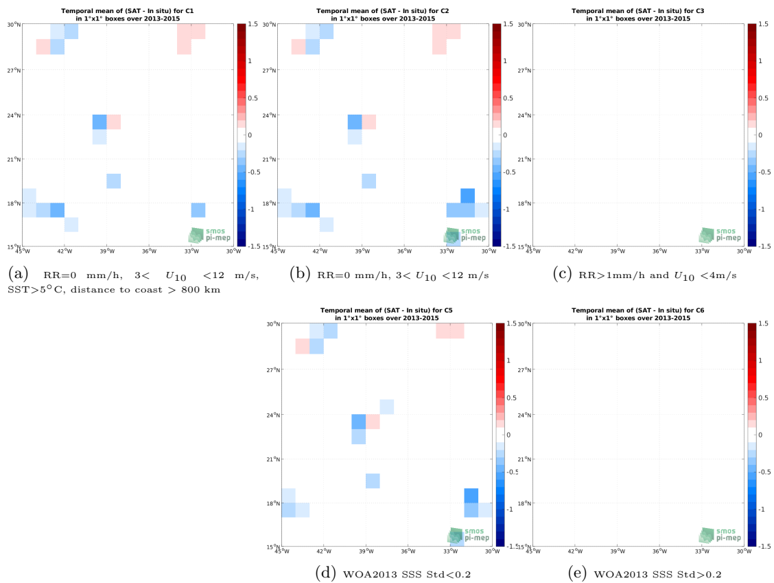
Figure 12: Temporal mean gridded over spatial boxes of size 1^\circ \times 1^\circ of \Delta SSS (Aquarius SSS L2 OR v5 (NASA-GSFC) - TSG (GOSUD-Sailing-ship)) for 5 different subdatasets corresponding to: RR=0 mm/h, 3 < U_{10} < 12 m/s, SST > 5^\circ C , distance to coast > 800 km (a), RR=0 mm/h, 3 < U_{10} < 12 m/s (b), RR > 1 mm/h and U_{10} < 4 m/s (c), WOA2013 SSS Std < 0.2 (d), WOA2013 SSS Std > 0.2 (e).
