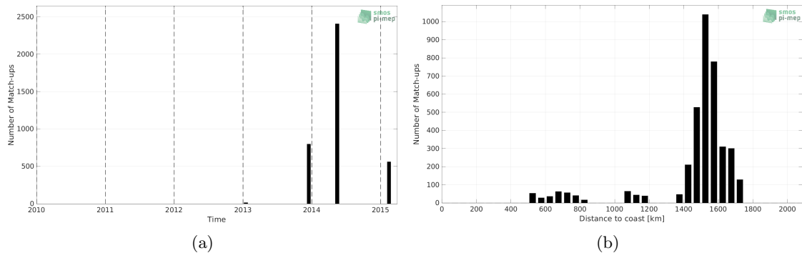
Figure 1: Number of match-ups between TSG (GOSUD-Sailing-ship) and Aquarius SSS L2 OR v5 (NASA-GSFC) SSS as a function of time (a) and as function of the distance to coast (b) over the SPURS 1 Pi-MEP region and for the full satellite product period.
