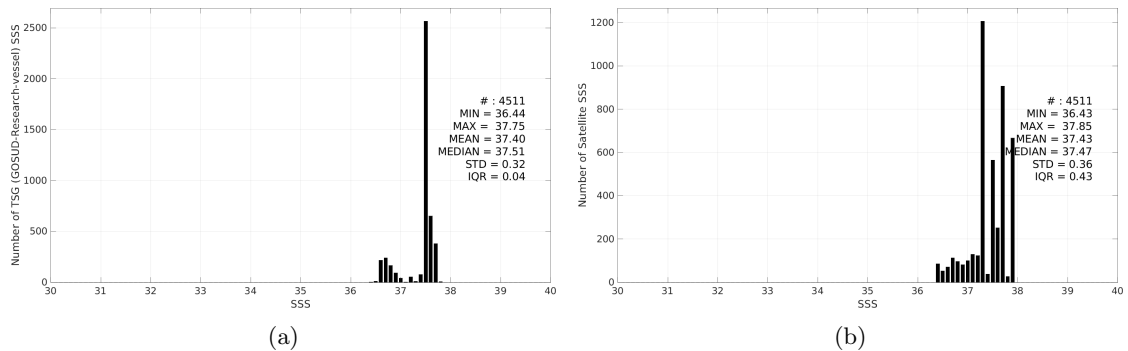
Figure 3: Histograms of SSS from TSG (GOSUD-Research-vessel) (a) and Aquarius SSS L2 OR v5 (NASA-GSFC) (b) considering all match-up pairs per bins of 0.1 over the SPURS 1 Pi-MEP region and for the full satellite product period.
