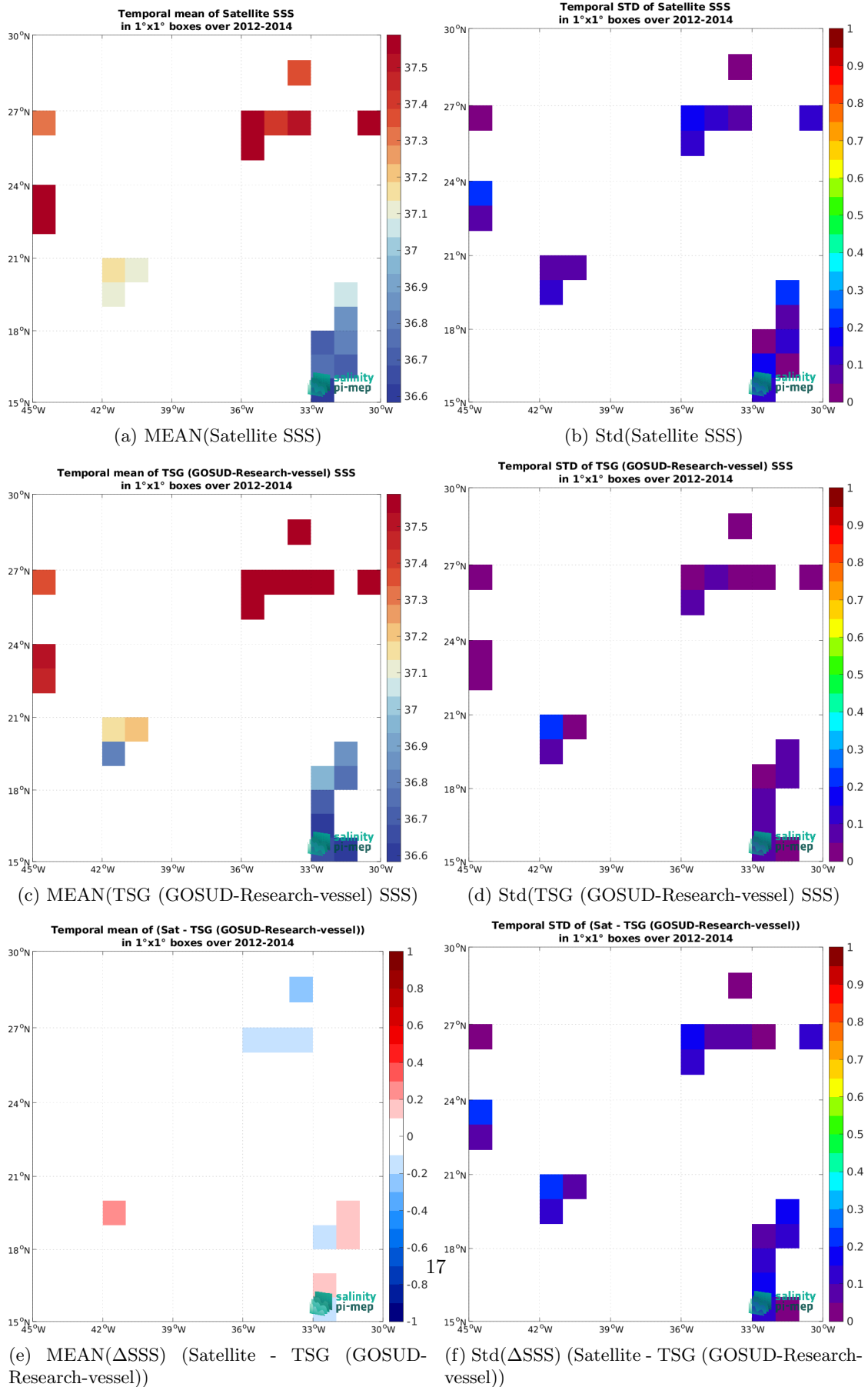
Figure 7: Temporal mean (left) and Std (right) of SSS from Aquarius SSS L2 OR v5 (NASA-GSFC) (top), TSG (GOSUD-Research-vessel) (middle), and of \Delta SSS (Satellite - TSG (GOSUD-Research-vessel)). Only match-up pairs are used to generate these maps.
