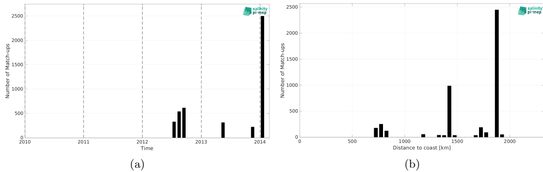
Figure 2: Number of match-ups between TSG (GOSUD-Research-vessel) and Aquarius SSS L2 OR v5 (NASA-GSFC) SSS as a function of time (a) and as function of the distance to coast (b) over the SPURS 1 Pi-MEP region and for the full satellite product period.
