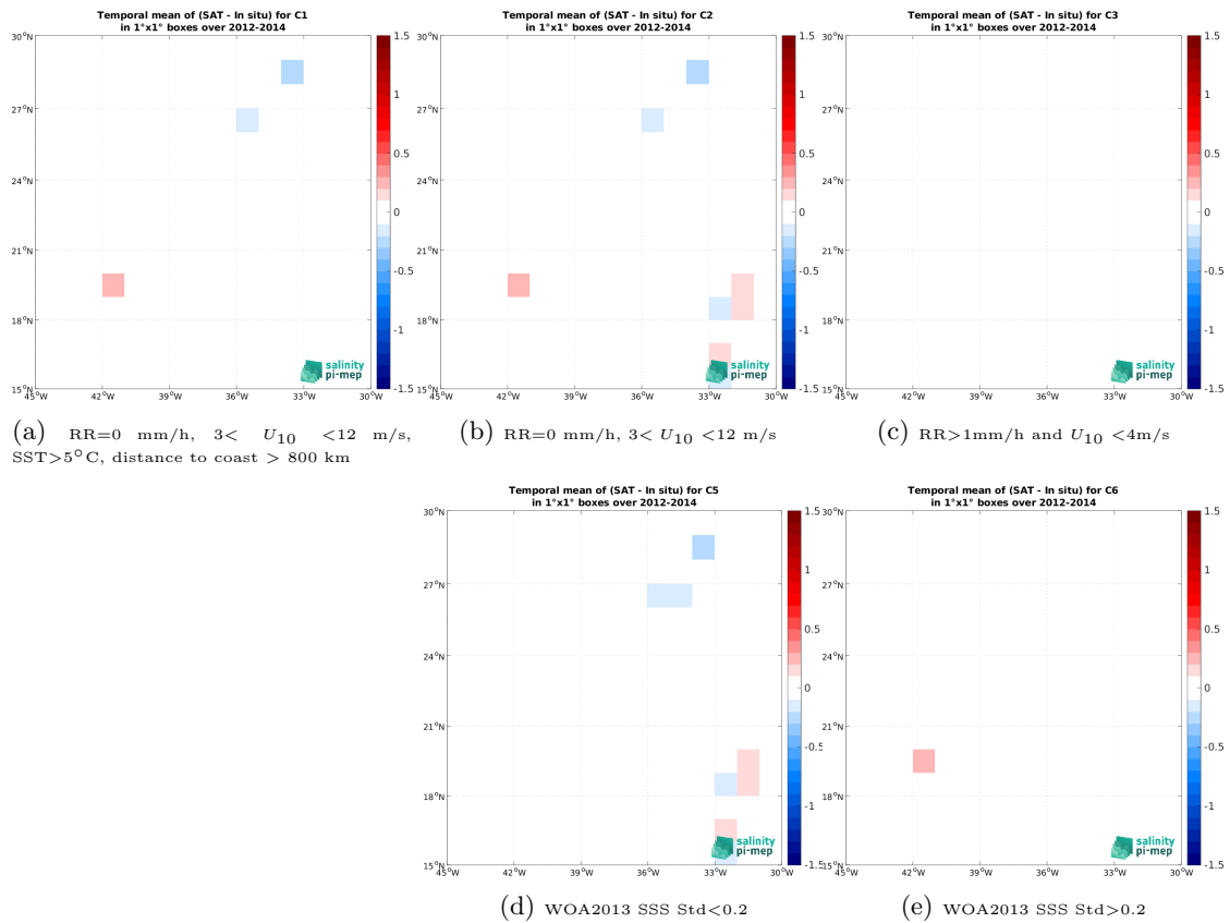
Figure 14: Temporal mean gridded over spatial boxes of size 1^\circ \times 1^\circ of \Delta SSS (Aquarius SSS L2 OR v5 (NASA-GSFC) - TSG (GOSUD-Research-vessel)) for 5 different subdatasets corresponding to:RR=0 mm/h, 3 < U_{10} < 12 m/s, SST>5°C, distance to coast > 800 km (a), RR=0 mm/h, 3 < U_{10} < 12 m/s (b), RR>1mm/h and U_{10} < 4 m/s (c), WOA2013 SSS Std<0.2 (d), WOA2013 SSS Std>0.2 (e).
