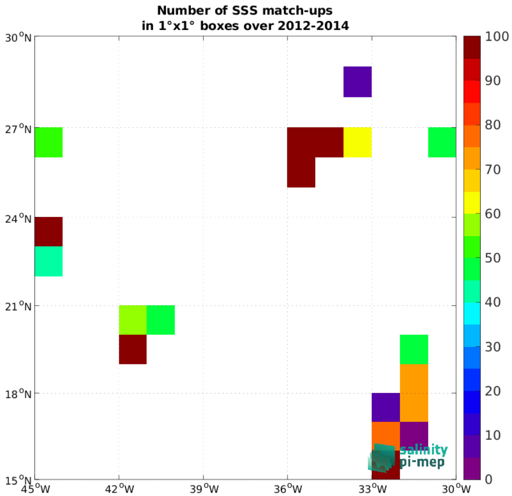
Figure 5: Number of SSS match-ups between TSG (GOSUD-Research-vessel) SSS and the Aquarius SSS L2 OR v5 (NASA-GSFC) SSS product for the SPURS 1 Pi-MEP region over 1°×1° boxes and for the full satellite product period.
