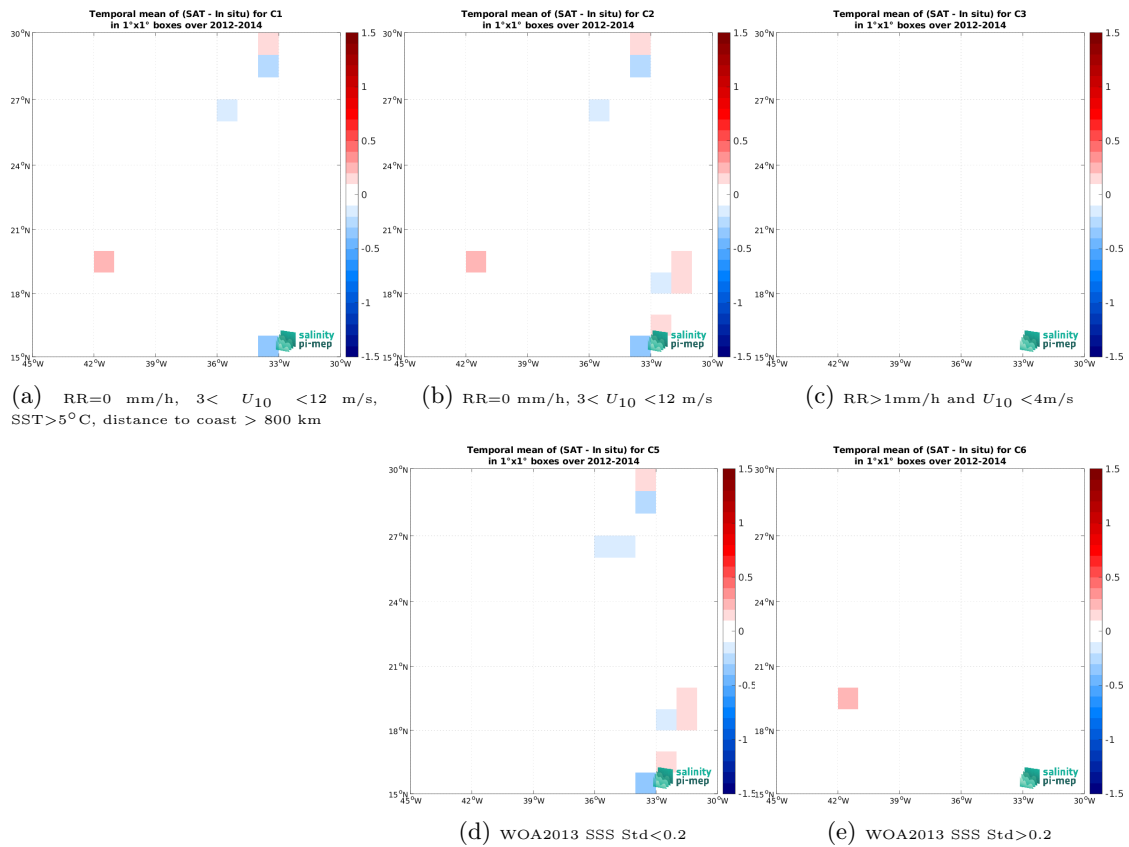
Figure 12: Temporal mean gridded over spatial boxes of size 1^\circ \times 1^\circ of \Delta SSS (Aquarius SSS L2 OR v5 (NASA-GSFC) - TSG (GOSUD-Research-vessel)) for 5 different subdatasets corresponding to:RR=0 mm/h, 3 < U_{10} < 12 m/s, SST>5°C, distance to coast > 800 km (a), RR=0 mm/h, 3 < U_{10} < 12 m/s (b), RR>1mm/h and U_{10} < 4 m/s (c), WOA2013 SSS Std<0.2 (d), WOA2013 SSS Std>0.2 (e).
