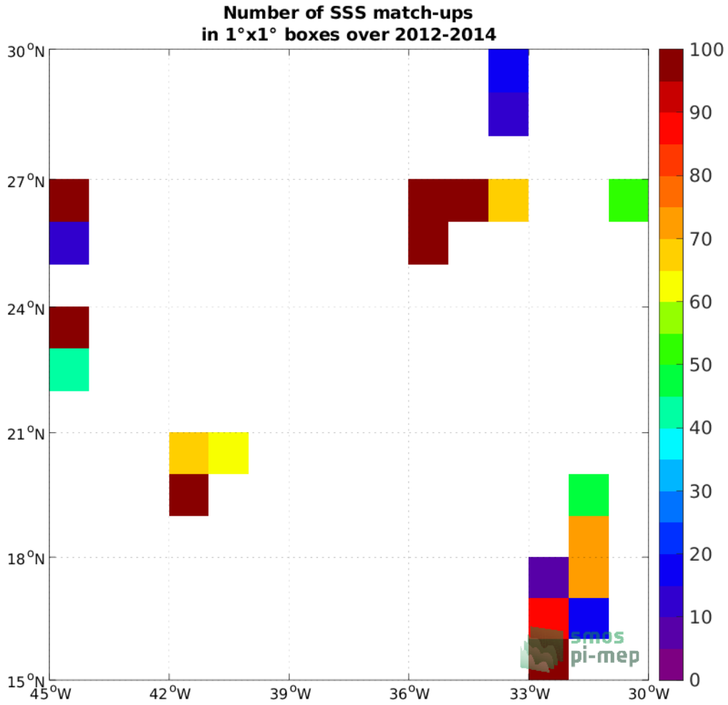
Figure 4: Number of SSS match-ups between TSG (GOSUD-Research-vessel) SSS and the Aquarius SSS L2 OR v5 (NASA-GSFC) SSS product for the SPURS 1 Pi-MEP region over 1°x1° boxes and for the full satellite product period.
