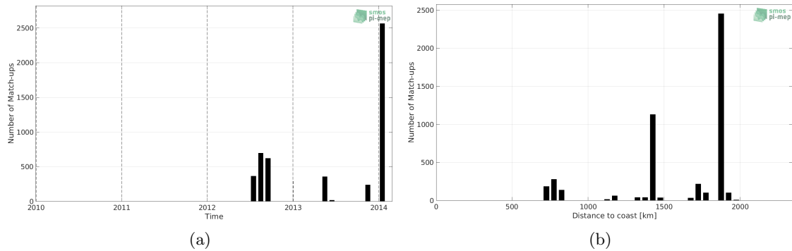
Figure 1: Number of match-ups between TSG (GOSUD-Research-vessel) and Aquarius SSS L2 OR v5 (NASA-GSFC) SSS as a function of time (a) and as function of the distance to coast (b) over the SPURS 1 Pi-MEP region and for the full satellite product period.
