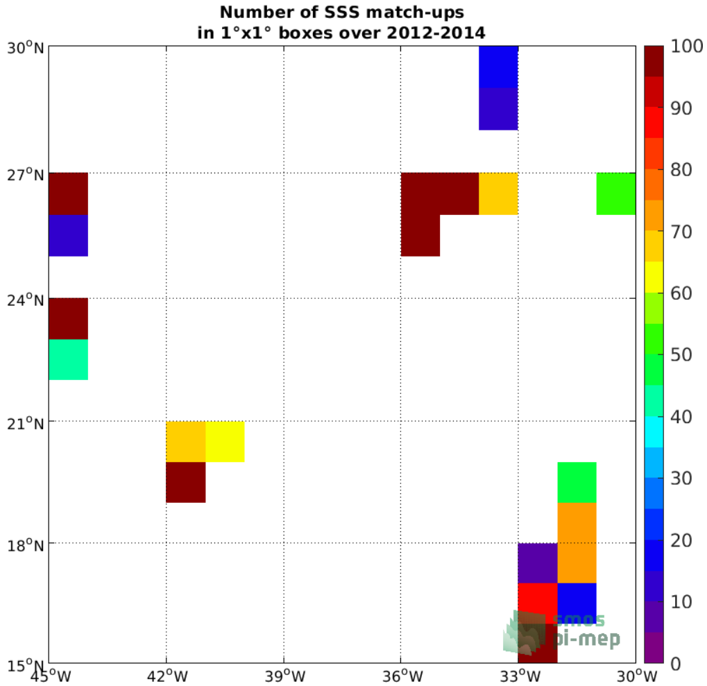
Figure 4: Number of SSS match-ups between TSG (GOSUD-Research-vessel) SSS and the Aquarius SSS L2 OR v5 (NASA-GSFC) SSS product for the SPURS 1 Pi-MEP region over 1^\circ \times 1^\circ boxes and for the full satellite product period.
