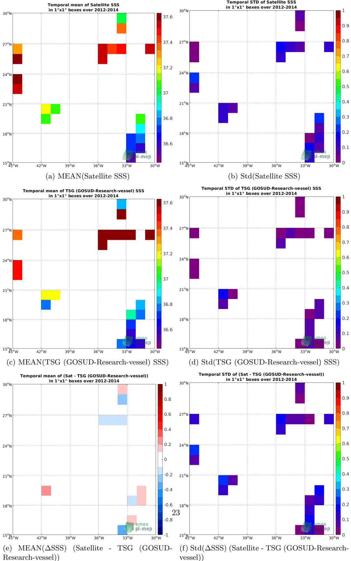
Figure 6: Temporal mean (left) and Std (right) of SSS from Aquarius SSS L2 OR v5 (NASA-GSFC) (top), TSG (GOSUD-Research-vessel) (middle), and of \Delta SSS (Satellite - TSG (GOSUD-Research-vessel)). Only match-up pairs are used to generate these maps.
