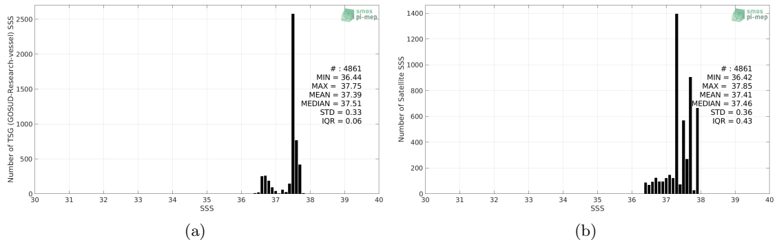
Figure 2: Histograms of SSS from TSG (GOSUD-Research-vessel) (a) and Aquarius SSS L2 OR v5 (NASA-GSFC) (b) considering all match-up pairs per bins of 0.1 over the SPURS 1 Pi-MEP region and for the full satellite product period.
