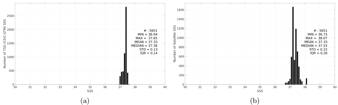
Figure 3: Histograms of SSS from TSG (CSIC-UTM) (a) and Aquarius SSS L2 OR v5 (NASA-GSFC) (b) considering all match-up pairs per bins of 0.1 over the SPURS 1 Pi-MEP region and for the full satellite product period.
