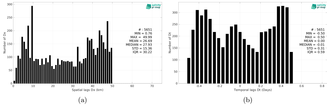
Figure 6: Histograms of the spatial (a) and temporal (b) lags between the location/time of the TSG (CSIC-UTM) measurement and the date of the corresponding Aquarius SSS L2 OR v5 (NASA-GSFC) SSS pixel.
