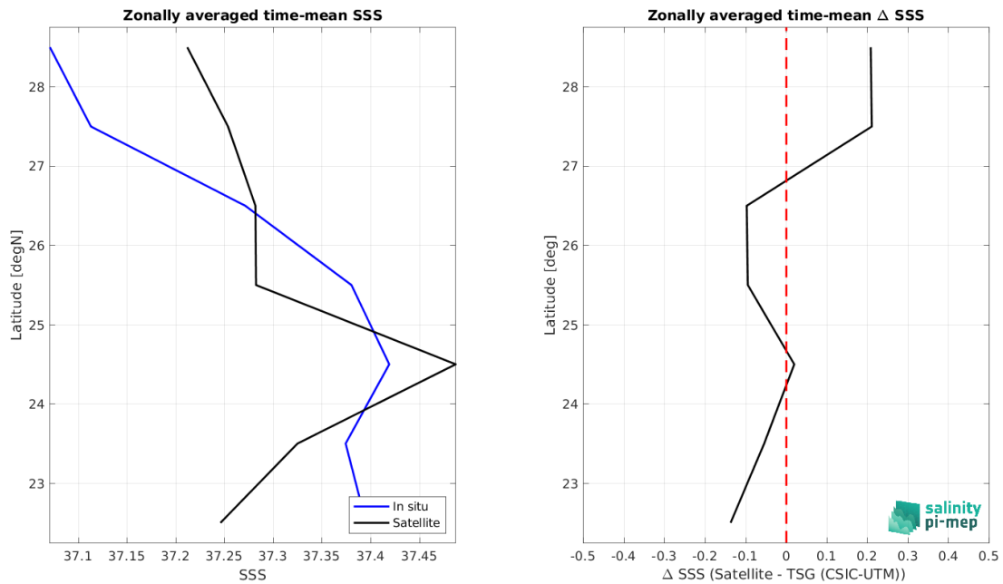
Figure 9: Left panel: Zonal mean SSS from Aquarius SSS L2 OR v5 (NASA-GSFC) satellite product (black) and from TSG (CSIC-UTM) (blue). Right panel: Zonal mean of \Delta SSS (Satellite - TSG (CSIC-UTM)) for all the collected Pi-MEP match-up pairs estimated over the full satellite product period.
