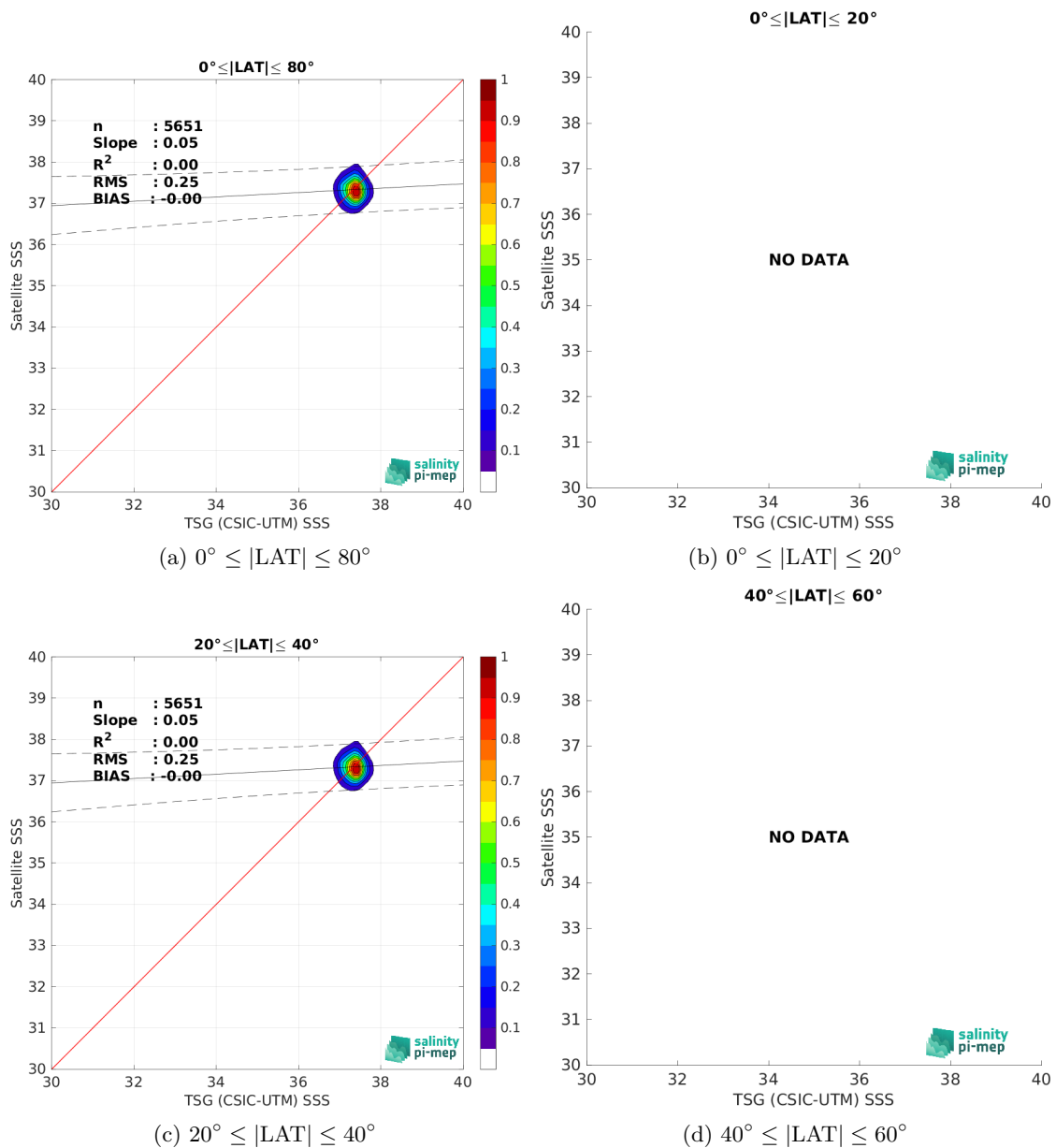
Figure 10: Contour maps of the concentration of Aquarius SSS L2 OR v5 (NASA-GSFC) SSS (y-axis) versus TSG (CSIC-UTM) SSS (x-axis) at match-up pairs for different latitude bands. For each plot, the red line shows x=y . The black thin and dashed lines indicate a linear fit through the data cloud and the \pm 95\% confidence levels, respectively. The number match-up pairs n , the slope and R^2 coefficient of the linear fit, the root mean square (RMS) and the mean bias between satellite and in situ data are indicated for each latitude band in each plots.
