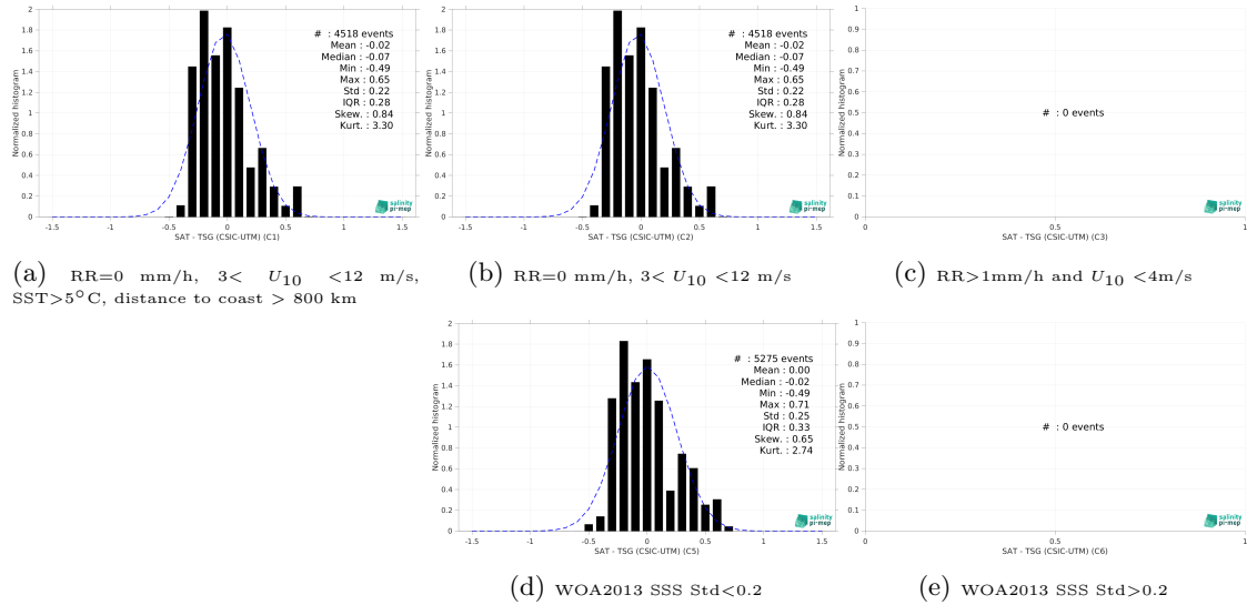
Figure 15: Normalized histogram of \Delta SSS (Aquarius SSS L2 OR v5 (NASA-GSFC) - TSG (CSIC-UTM)) for 5 different subdatasets corresponding to: RR=0 mm/h, 3 < U_{10} < 12 m/s, SST>5°C, distance to coast > 800 km (a), RR=0 mm/h, 3 < U_{10} < 12 m/s (b), RR>1mm/h and U_{10} < 4 m/s (c), WOA2013 SSS Std<0.2 (d), WOA2013 SSS Std>0.2 (e).
