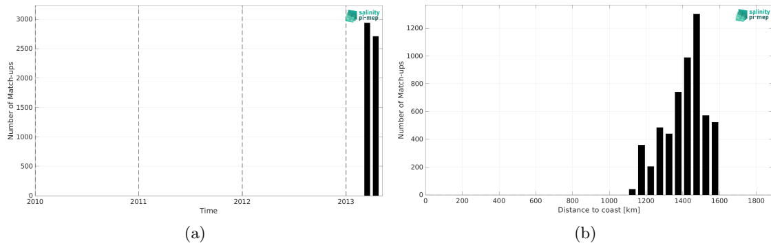
Figure 2: Number of match-ups between TSG (CSIC-UTM) and Aquarius SSS L2 OR v5 (NASA-GSFC) SSS as a function of time (a) and as function of the distance to coast (b) over the SPURS 1 Pi-MEP region and for the full satellite product period.
