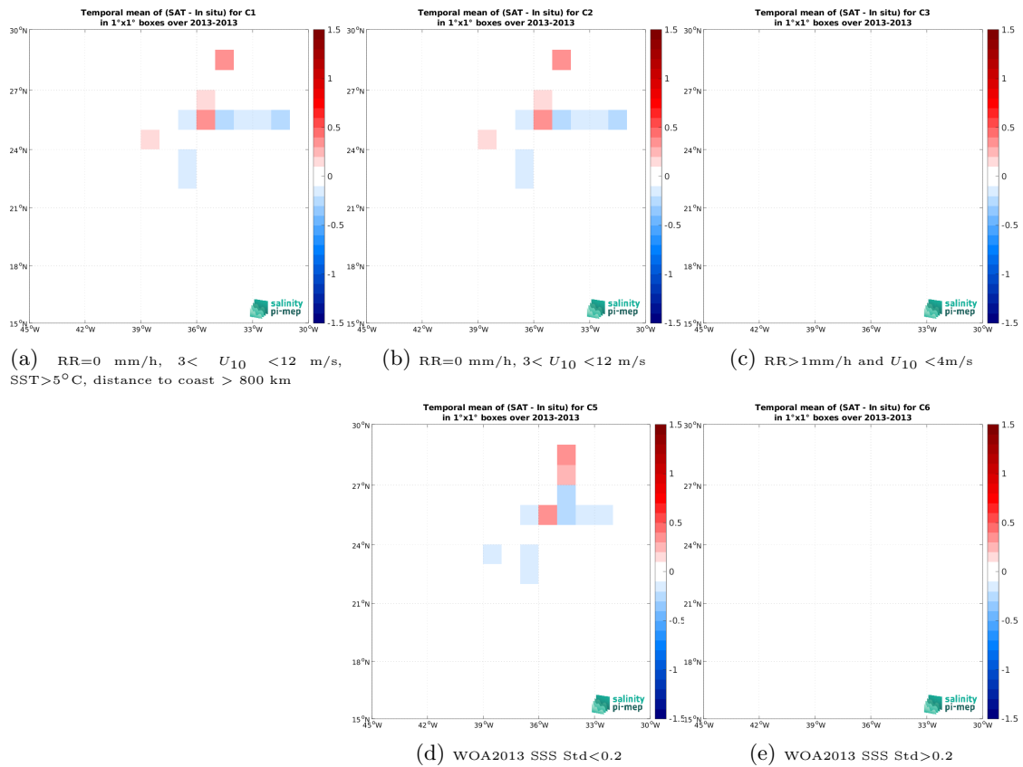
Figure 14: Temporal mean gridded over spatial boxes of size 1^\circ \times 1^\circ of \Delta SSS (Aquarius SSS L2 OR v5 (NASA-GSFC) - TSG (CSIC-UTM)) for 5 different subdatasets corresponding to: RR=0 mm/h, 3 < U_{10} < 12 m/s, SST > 5^\circ C , distance to coast > 800 km (a), RR=0 mm/h, 3 < U_{10} < 12 m/s (b), RR > 1 mm/h and U_{10} < 4 m/s (c), WOA2013 SSS Std < 0.2 (d), WOA2013 SSS Std > 0.2 (e).
