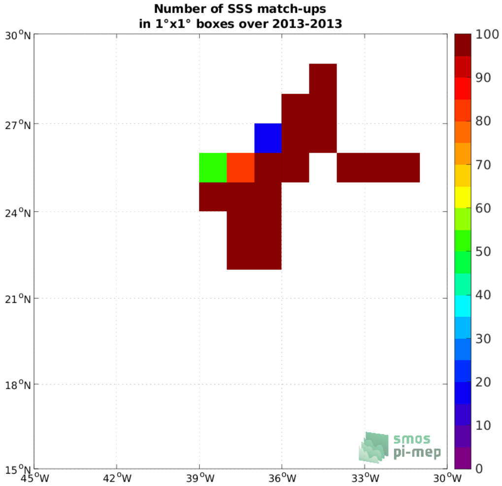
Figure 4: Number of SSS match-ups between TSG (CSIC-UTM) SSS and the Aquarius SSS L2 OR v5 (NASA-GSFC) SSS product for the SPURS 1 Pi-MEP region over 1^\circ \times 1^\circ boxes and for the full satellite product period.
