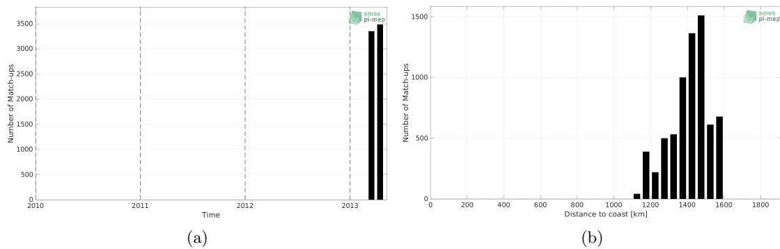
Figure 1: Number of match-ups between TSG (CSIC-UTM) and Aquarius SSS L2 OR v5 (NASA-GSFC) SSS as a function of time (a) and as function of the distance to coast (b) over the SPURS 1 Pi-MEP region and for the full satellite product period.
