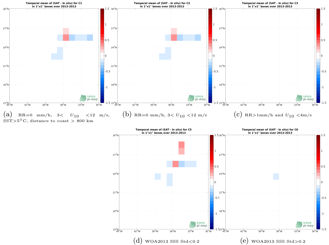
Figure 12: Temporal mean gridded over spatial boxes of size 1^{\circ}\times 1^{\circ} of \Delta\text{SSS} (Aquarius SSS L2 OR v5 (NASA-GSFC) - TSG (CSIC-UTM)) for 5 different subdatasets corresponding to:RR=0 mm/h, 3 < U_{10} < 12 m/s, SST >5^{\circ}\text{C} , distance to coast > 800 km (a), RR=0 mm/h, 3 < U_{10} < 12 m/s (b), RR >1 mm/h and U_{10} < 4 m/s (c), WOA2013 SSS Std <0.2 (d), WOA2013 SSS Std >0.2 (e).
