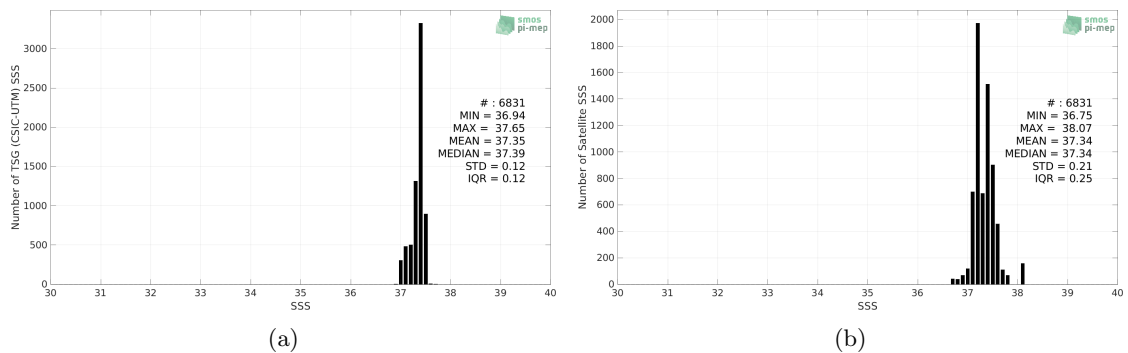
Figure 2: Histograms of SSS from TSG (CSIC-UTM) (a) and Aquarius SSS L2 OR v5 (NASA-GSFC) (b) considering all match-up pairs per bins of 0.1 over the SPURS 1 Pi-MEP region and for the full satellite product period.
