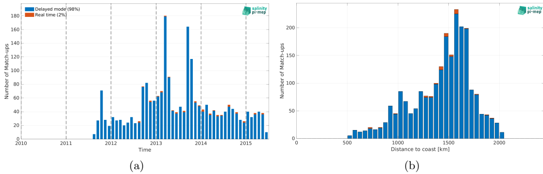
Figure 1: Number of match-ups between Argo and Aquarius SSS L2 OR v5 (NASA-GSFC) SSS as a function of time (a) and as function of the distance to coast (b) over the SPURS 1 Pi-MEP region and for the full satellite product period.
