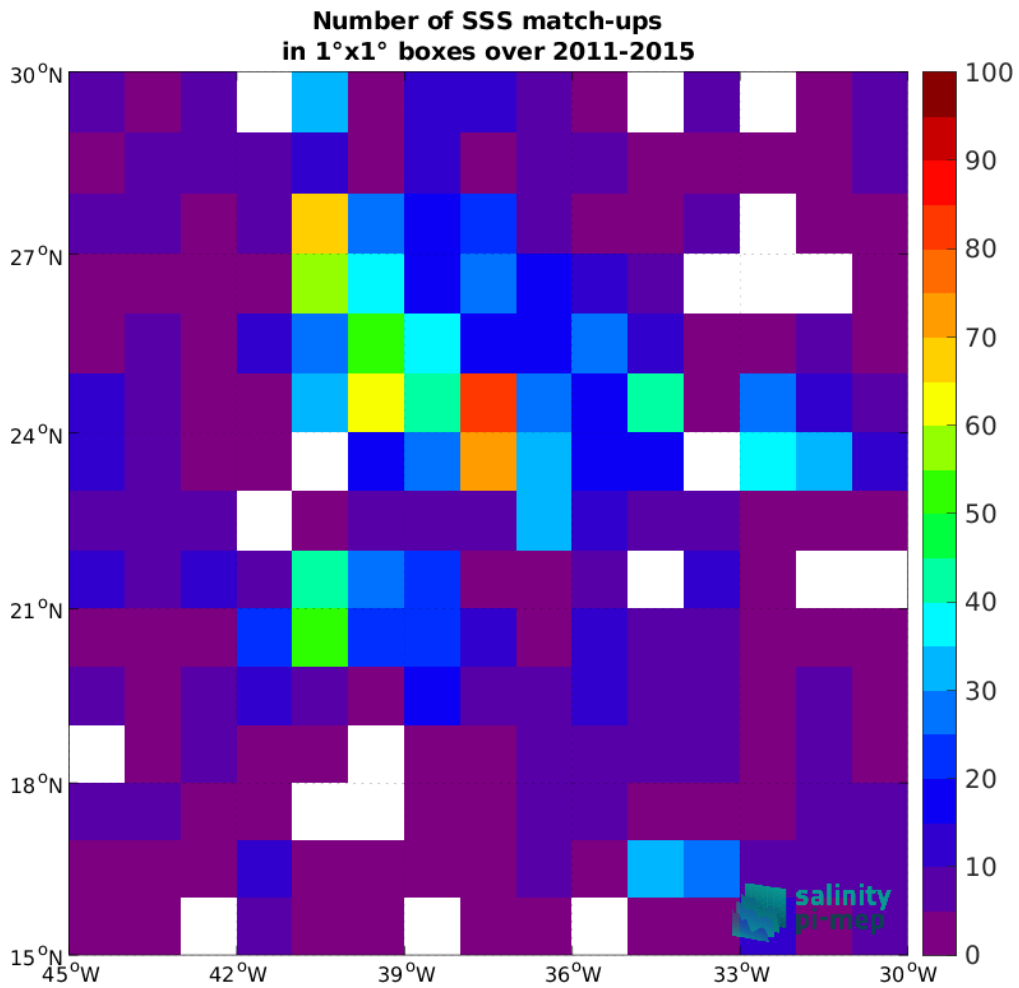
Figure 4: Number of SSS match-ups between Argo SSS and the Aquarius SSS L2 OR v5 (NASA-GSFC) SSS product for the SPURS 1 Pi-MEP region over 1^\circ \times 1^\circ boxes and for the full satellite product period.
