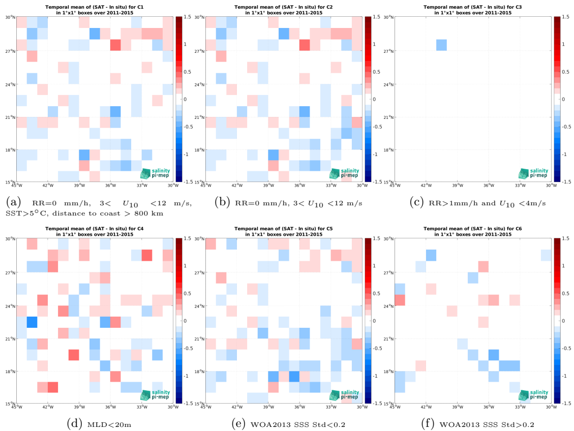
Figure 12: Temporal mean gridded over spatial boxes of size 1^\circ \times 1^\circ of \Delta SSS (Aquarius SSS L2 OR v5 (NASA-GSFC) - Argo) for 6 different subdatasets corresponding to: RR=0 mm/h, 3 < U_{10} < 12 m/s, SST > 5^\circ\text{C} , distance to coast > 800 km (a), RR=0 mm/h, 3 < U_{10} < 12 m/s (b), RR > 1 mm/h and U_{10} < 4 m/s (c), MLD < 20 m (d), WOA2013 SSS Std < 0.2 (e), WOA2013 SSS Std > 0.2 (f).
