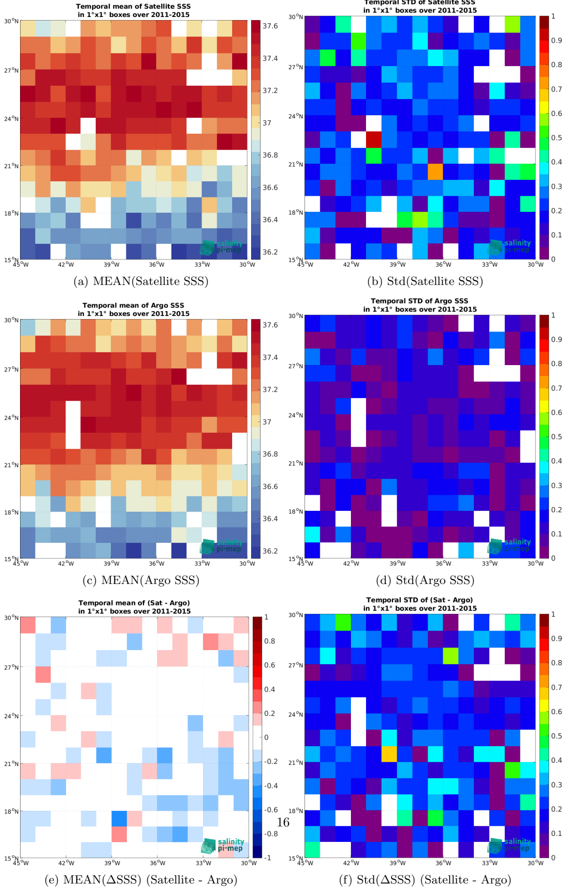
Figure 6: Temporal mean (left) and Std (right) of SSS from Aquarius SSS L2 OR v5 (NASA-GSFC) (top), Argo (middle), and of \Delta SSS (Satellite - Argo). Only match-up pairs are used to generate these maps.
