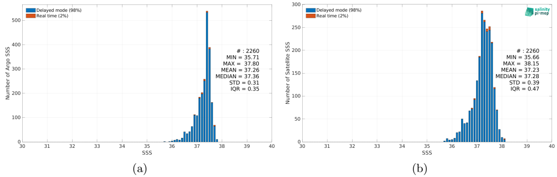
Figure 2: Histograms of SSS from Argo (a) and Aquarius SSS L2 OR v5 (NASA-GSFC) (b) considering all match-up pairs per bins of 0.1 over the SPURS 1 Pi-MEP region and for the full satellite product period.
