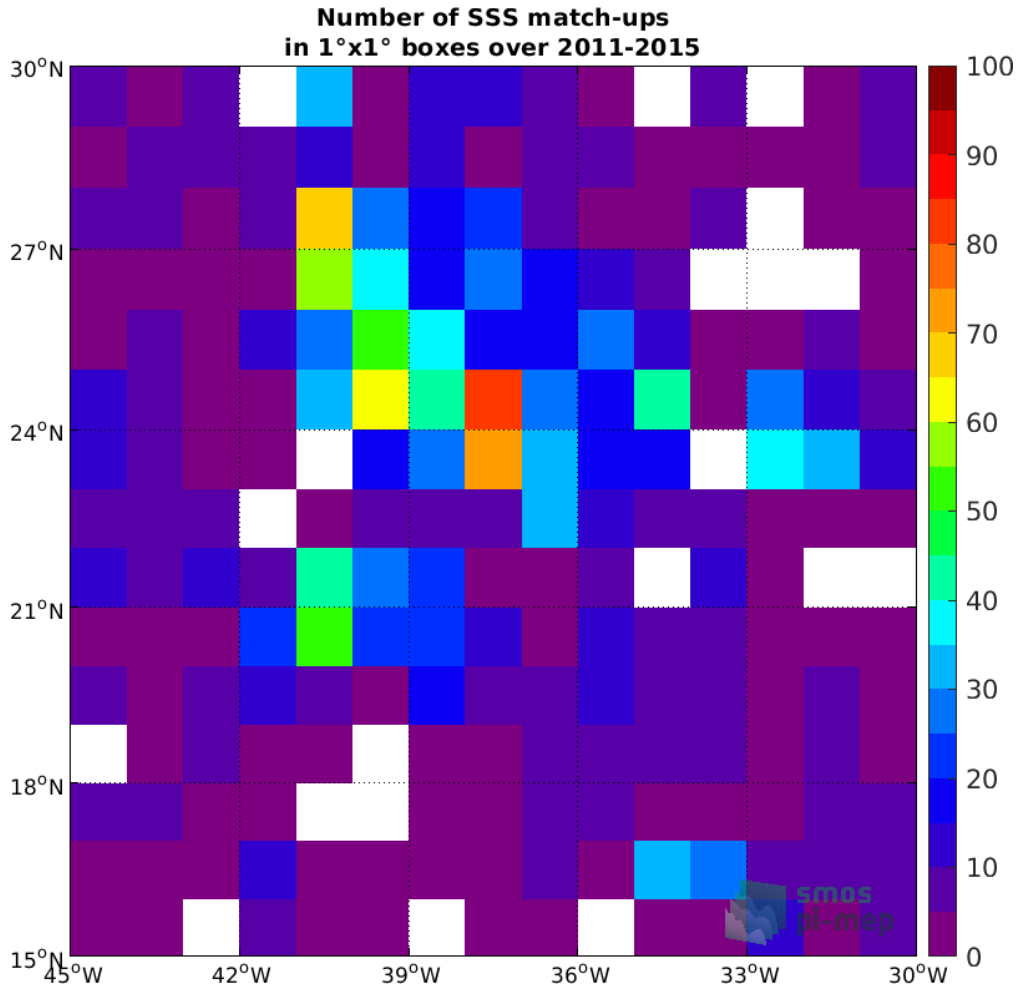
Figure 4: Number of SSS match-ups between Argo SSS and the Aquarius SSS L2 OR v5 (NASA-GSFC) SSS product for the SPURS 1 Pi-MEP region over 1°x1° boxes and for the full satellite product period.
