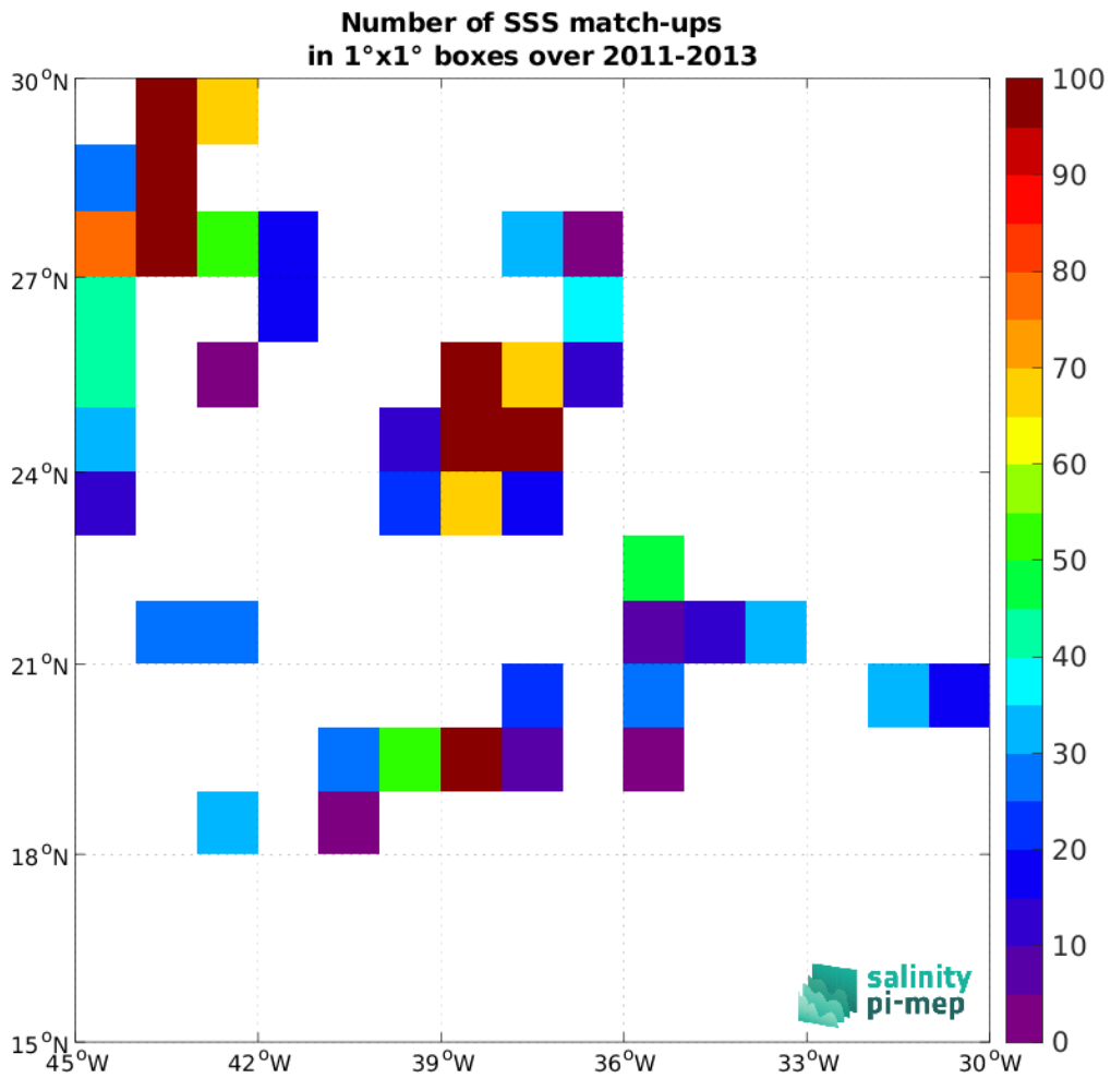
Figure 5: Number of SSS match-ups between TSG (SAMOS) SSS and the Aquarius SSS L2 CAP v5 (JPL) SSS product for the SPURS 1 Pi-MEP region over 1^\circ \times 1^\circ boxes and for the full satellite product period.
