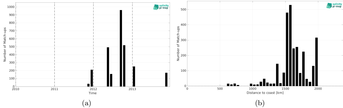
Figure 2: Number of match-ups between TSG (SAMOS) and Aquarius SSS L2 CAP v5 (JPL) SSS as a function of time (a) and as function of the distance to coast (b) over the SPURS 1 Pi-MEP region and for the full satellite product period.
