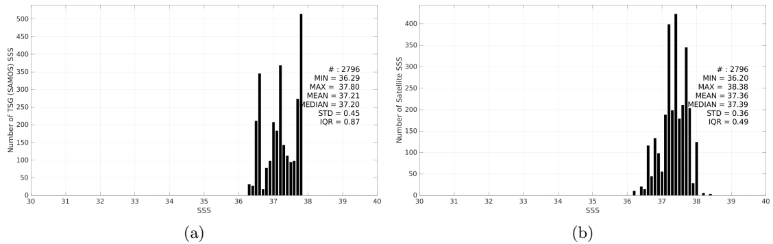
Figure 3: Histograms of SSS from TSG (SAMOS) (a) and Aquarius SSS L2 CAP v5 (JPL) (b) considering all match-up pairs per bins of 0.1 over the SPURS 1 Pi-MEP region and for the full satellite product period.
