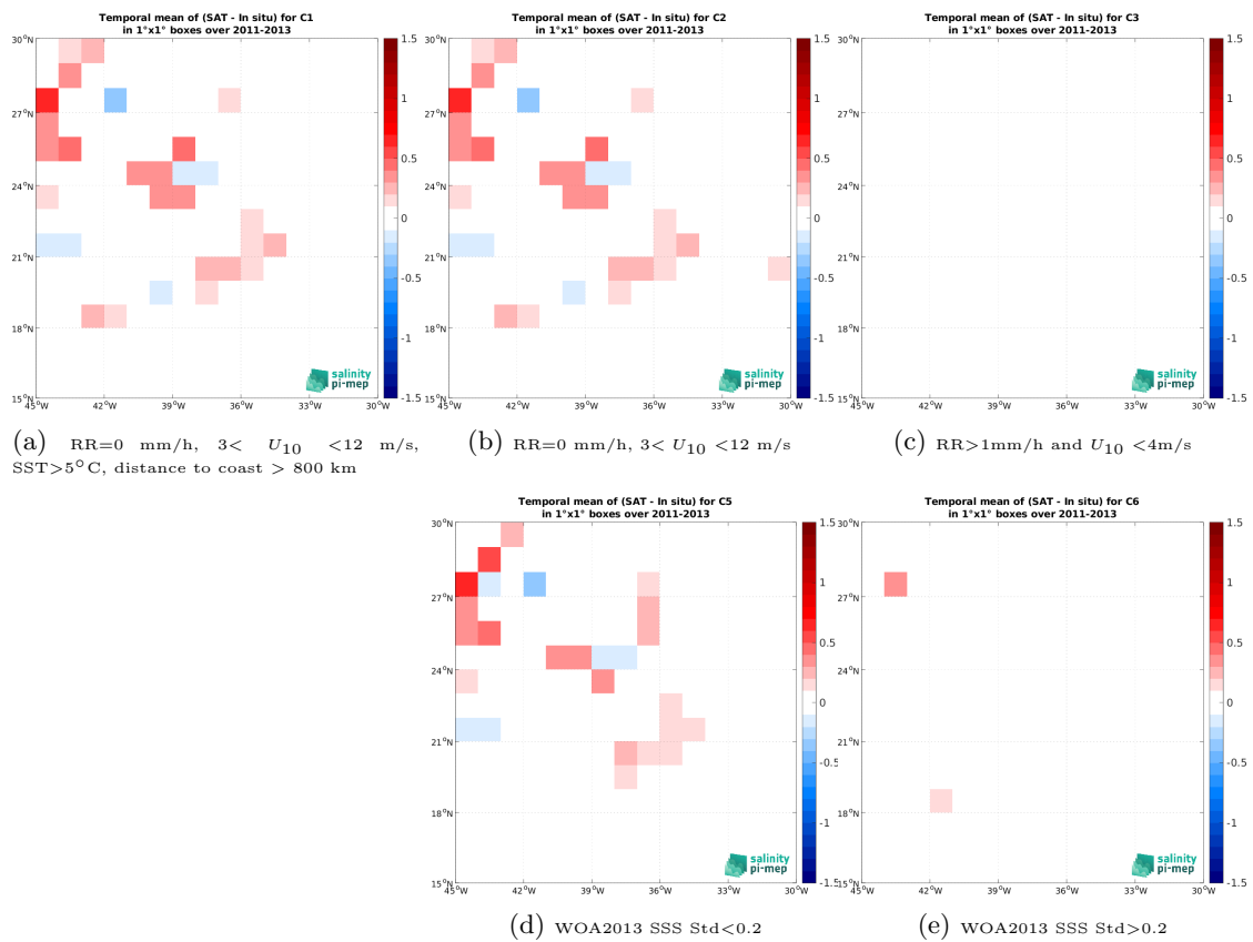
Figure 14: Temporal mean gridded over spatial boxes of size 1^\circ \times 1^\circ of \Delta\text{SSS} (Aquarius SSS L2 CAP v5 (JPL) - TSG (SAMOS)) for 5 different subdatasets corresponding to:RR=0 mm/h, 3 < U_{10} < 12 m/s, SST>5°C, distance to coast > 800 km (a), RR=0 mm/h, 3 < U_{10} < 12 m/s (b), RR>1mm/h and U_{10} < 4 m/s (c), WOA2013 SSS Std<0.2 (d), WOA2013 SSS Std>0.2 (e).
