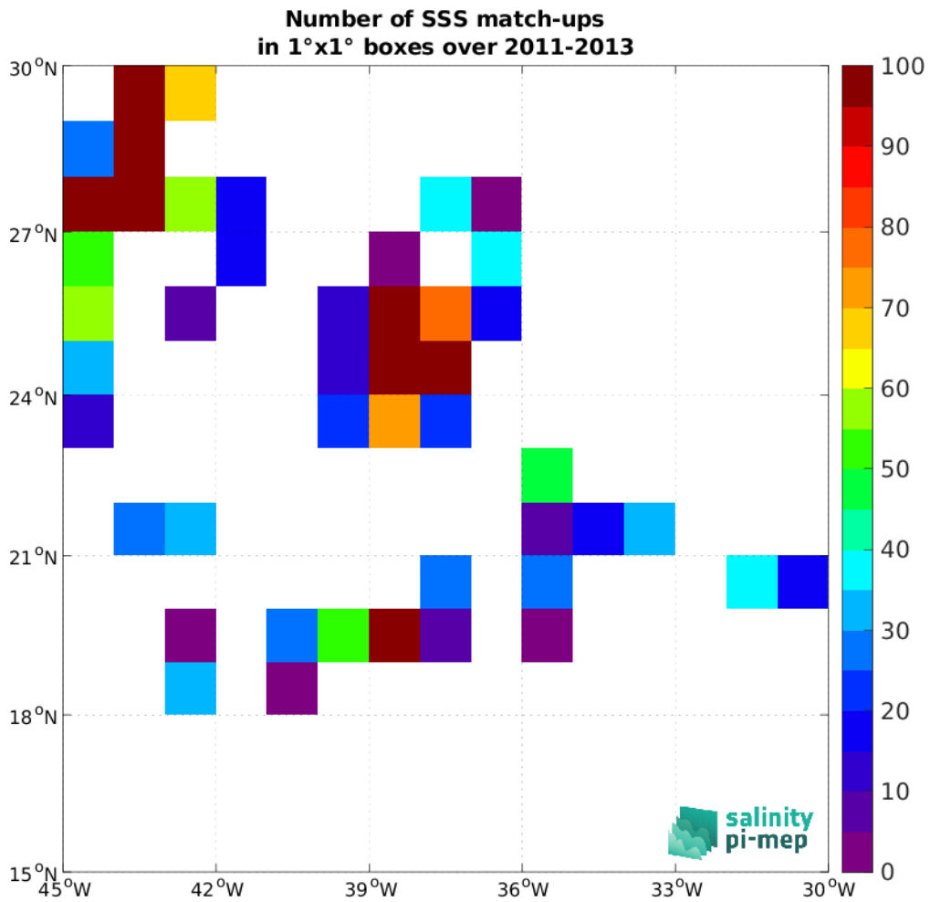
Figure 4: Number of SSS match-ups between TSG (SAMOS) SSS and the Aquarius SSS L2 CAP v5 (JPL) SSS product for the SPURS 1 Pi-MEP region over 1^\circ \times 1^\circ boxes and for the full satellite product period.
