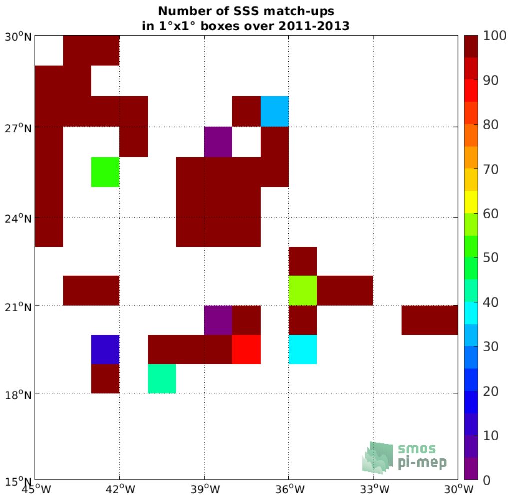
Figure 4: Number of SSS match-ups between TSG (SAMOS) SSS and the Aquarius SSS L2 CAP v5 (JPL) SSS product for the SPURS 1 Pi-MEP region over 1^\circ \times 1^\circ boxes and for the full satellite product period.
