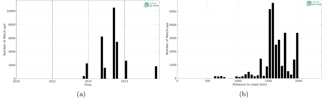
Figure 1: Number of match-ups between TSG (SAMOS) and Aquarius SSS L2 CAP v5 (JPL) SSS as a function of time (a) and as function of the distance to coast (b) over the SPURS 1 Pi-MEP region and for the full satellite product period.
