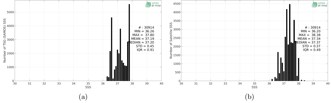
Figure 2: Histograms of SSS from TSG (SAMOS) (a) and Aquarius SSS L2 CAP v5 (JPL) (b) considering all match-up pairs per bins of 0.1 over the SPURS 1 Pi-MEP region and for the full satellite product period.
