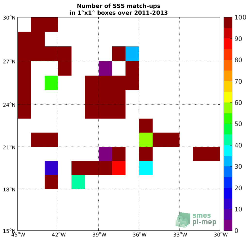
Figure 4: Number of SSS match-ups between TSG (SAMOS) SSS and the Aquarius SSS L2 CAP v5 (JPL) SSS product for the SPURS 1 Pi-MEP region over 1°x1° boxes and for the full satellite product period.
