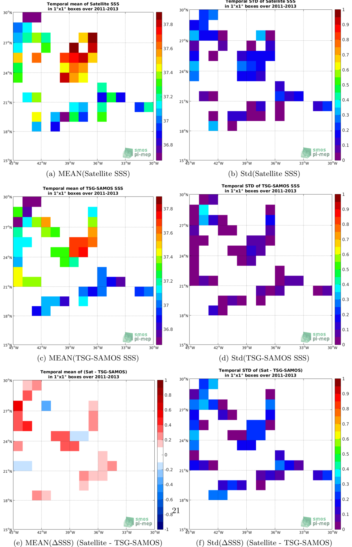
Figure 6: Temporal mean (left) and Std (right) of SSS from Aquarius-L2-JPL-V5 (top), TSG-SAMOS (middle), and of \Delta SSS (Satellite - TSG-SAMOS). Only match-up pairs are used to generate these maps.
