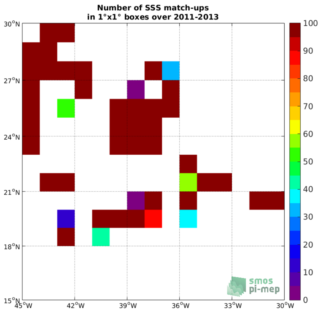
Figure 4: Number of SSS match-ups between TSG-SAMOS SSS and the Aquarius-L2-JPL-V5 SSS product for the SPURS 1 Pi-MEP region over 1°x1° boxes and for the full satellite product period.
