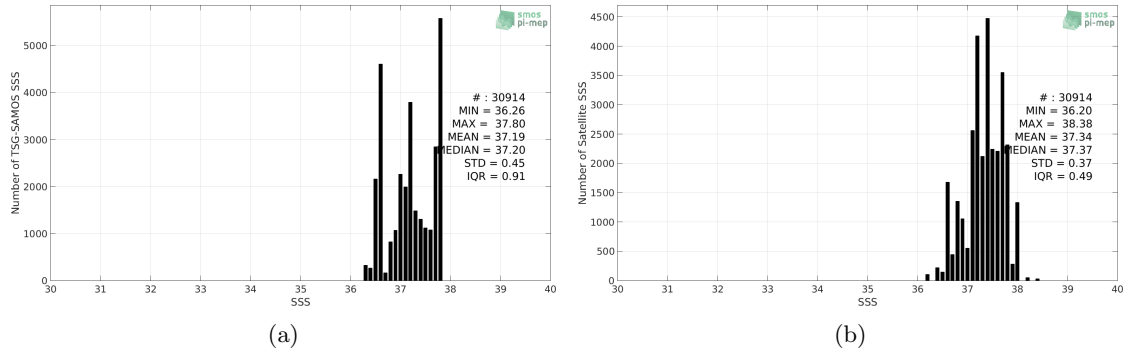
Figure 2: Histograms of SSS from TSG-SAMOS (a) and Aquarius-L2-JPL-V5 (b) considering all match-up pairs per bins of 0.1 over the SPURS 1 Pi-MEP region and for the full satellite product period.
