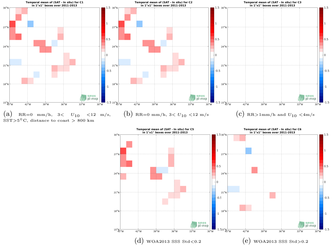
Figure 12: Temporal mean gridded over spatial boxes of size 1^\circ \times 1^\circ of \Delta SSS (Aquarius-L2-JPL-V5 - TSG-SAMOS) for 5 different subdatasets corresponding to: RR=0 mm/h, 3 < U_{10} < 12 m/s, SST > 5^\circ C , distance to coast > 800 km (a), RR=0 mm/h, 3 < U_{10} < 12 m/s (b), RR > 1 mm/h and U_{10} < 4 m/s (c), WOA2013 SSS Std < 0.2 (d), WOA2013 SSS Std > 0.2 (e).
