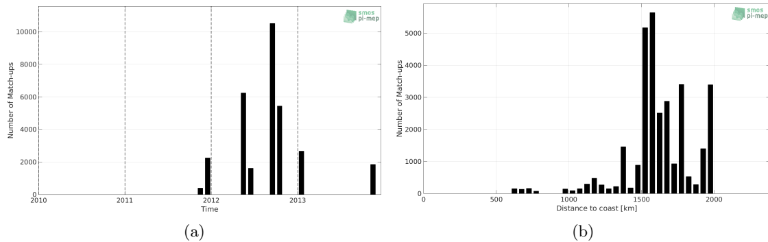
Figure 1: Number of match-ups between TSG-SAMOS and Aquarius-L2-JPL-V5 SSS as a function of time (a) and as function of the distance to coast (b) over the SPURS 1 Pi-MEP region and for the full satellite product period.
