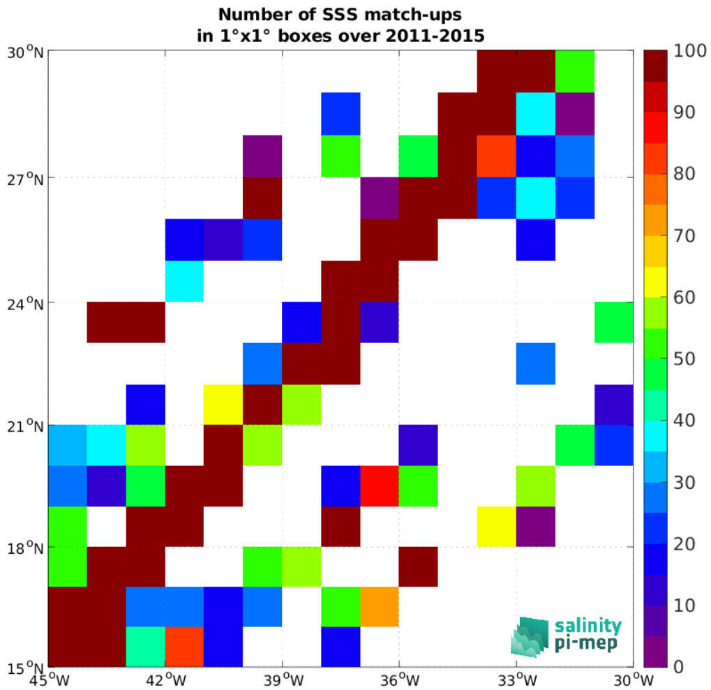
Figure 5: Number of SSS match-ups between TSG (LEGOS-DM) SSS and the Aquarius SSS L2 CAP v5 (JPL) SSS product for the SPURS 1 Pi-MEP region over 1^\circ \times 1^\circ boxes and for the full satellite product period.
