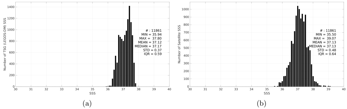
Figure 3: Histograms of SSS from TSG (LEGOS-DM) (a) and Aquarius SSS L2 CAP v5 (JPL) (b) considering all match-up pairs per bins of 0.1 over the SPURS 1 Pi-MEP region and for the full satellite product period.
