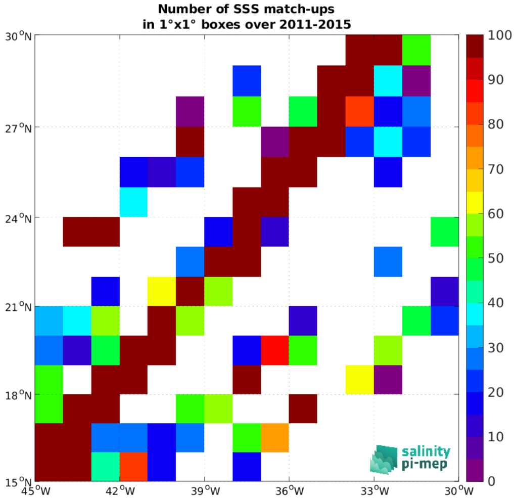
Figure 5: Number of SSS match-ups between TSG (LEGOS-DM) SSS and the Aquarius SSS L2 CAP v5 (JPL) SSS product for the SPURS 1 Pi-MEP region over 1°x1° boxes and for the full satellite product period.
