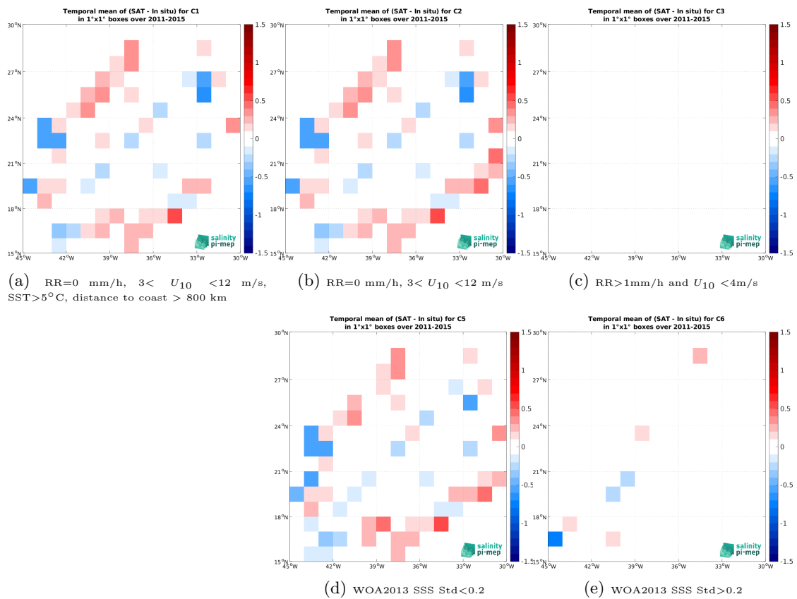
Figure 14: Temporal mean gridded over spatial boxes of size 1^\circ \times 1^\circ of \Delta\text{SSS} (Aquarius SSS L2 CAP v5 (JPL) - TSG (LEGOS-DM)) for 5 different subdatasets corresponding to:RR=0 mm/h, 3 < U_{10} < 12 m/s, SST>5°C, distance to coast > 800 km (a), RR=0 mm/h, 3 < U_{10} < 12 m/s (b), RR>1mm/h and U_{10} < 4 m/s (c), WOA2013 SSS Std<0.2 (d), WOA2013 SSS Std>0.2 (e).
