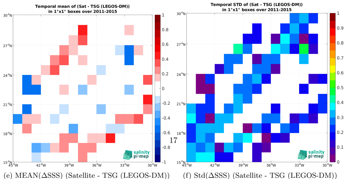
Figure 6: Temporal mean (left) and Std (right) of SSS from Aquarius SSS L2 CAP v5 (JPL) (top), TSG (LEGOS-DM) (middle), and of \Delta SSS (Satellite - TSG (LEGOS-DM)). Only match-up pairs are used to generate these maps.
