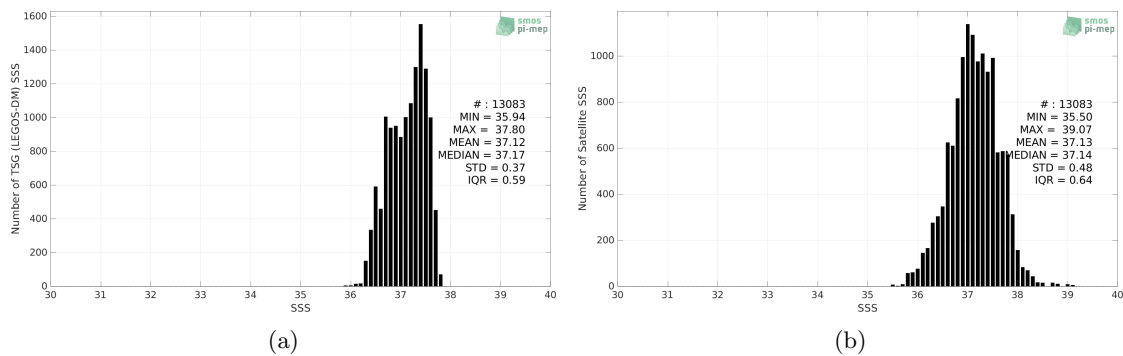
Figure 2: Histograms of SSS from TSG (LEGOS-DM) (a) and Aquarius SSS L2 CAP v5 (JPL) (b) considering all match-up pairs per bins of 0.1 over the SPURS 1 Pi-MEP region and for the full satellite product period.
