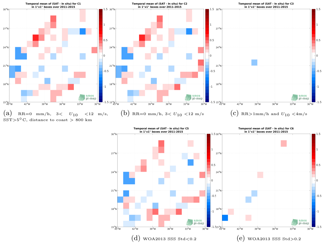
Figure 12: Temporal mean gridded over spatial boxes of size 1^\circ \times 1^\circ of \Delta\text{SSS} (Aquarius SSS L2 CAP v5 (JPL) - TSG (LEGOS-DM)) for 5 different subdatasets corresponding to:RR=0 mm/h, 3 < U_{10} < 12 m/s, SST >5^\circ\text{C} , distance to coast > 800 km (a), RR=0 mm/h, 3 < U_{10} < 12 m/s (b), RR >1 mm/h and U_{10} < 4 m/s (c), WOA2013 SSS Std <0.2 (d), WOA2013 SSS Std >0.2 (e).
