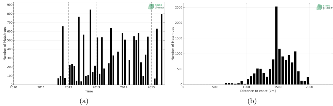
Figure 1: Number of match-ups between TSG (LEGOS-DM) and Aquarius SSS L2 CAP v5 (JPL) SSS as a function of time (a) and as function of the distance to coast (b) over the SPURS 1 Pi-MEP region and for the full satellite product period.
