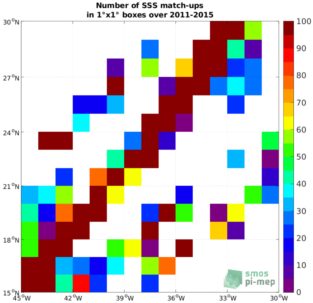
Figure 4: Number of SSS match-ups between TSG (LEGOS-DM) SSS and the Aquarius SSS L2 CAP v5 (JPL) SSS product for the SPURS 1 Pi-MEP region over 1°x1° boxes and for the full satellite product period.
