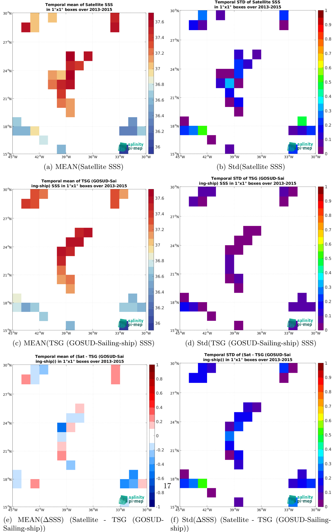
Figure 7: Temporal mean (left) and Std (right) of SSS from Aquarius SSS L2 CAP v5 (JPL) (top), TSG (GOSUD-Sailing-ship) (middle), and of \Delta SSS (Satellite - TSG (GOSUD-Sailing-ship)). Only match-up pairs are used to generate these maps.
