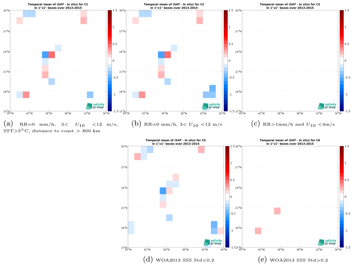
Figure 14: Temporal mean gridded over spatial boxes of size 1^\circ \times 1^\circ of \Delta SSS (Aquarius SSS L2 CAP v5 (JPL) - TSG (GOSUD-Sailing-ship)) for 5 different subdatasets corresponding to: RR=0 mm/h, 3 < U_{10} < 12 m/s, SST > 5^\circ C , distance to coast > 800 km (a), RR=0 mm/h, 3 < U_{10} < 12 m/s (b), RR > 1 mm/h and U_{10} < 4 m/s (c), WOA2013 SSS Std <0.2 (d), WOA2013 SSS Std >0.2 (e).
