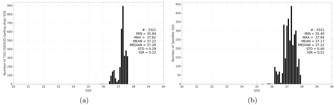
Figure 3: Histograms of SSS from TSG (GOSUD-Sailing-ship) (a) and Aquarius SSS L2 CAP v5 (JPL) (b) considering all match-up pairs per bins of 0.1 over the SPURS 1 Pi-MEP region and for the full satellite product period.
