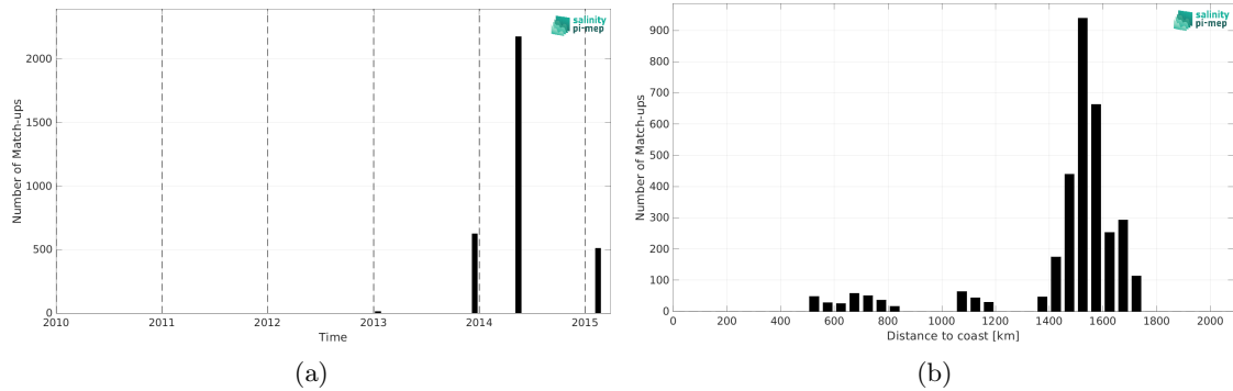
Figure 2: Number of match-ups between TSG (GOSUD-Sailing-ship) and Aquarius SSS L2 CAP v5 (JPL) SSS as a function of time (a) and as function of the distance to coast (b) over the SPURS 1 Pi-MEP region and for the full satellite product period.
