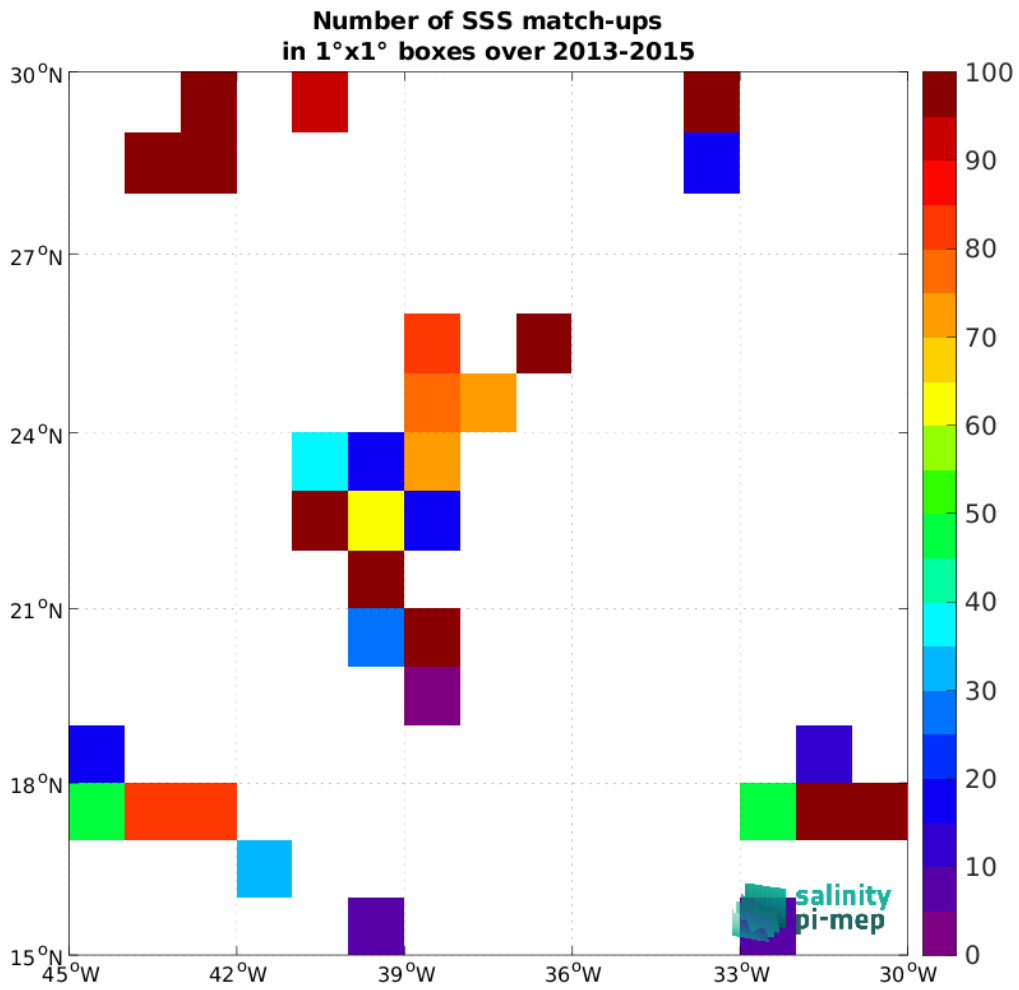
Figure 5: Number of SSS match-ups between TSG (GOSUD-Sailing-ship) SSS and the Aquarius SSS L2 CAP v5 (JPL) SSS product for the SPURS 1 Pi-MEP region over 1°x1° boxes and for the full satellite product period.
