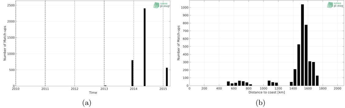
Figure 1: Number of match-ups between TSG (GOSUD-Sailing-ship) and Aquarius SSS L2 CAP v5 (JPL) SSS as a function of time (a) and as function of the distance to coast (b) over the SPURS 1 Pi-MEP region and for the full satellite product period.
