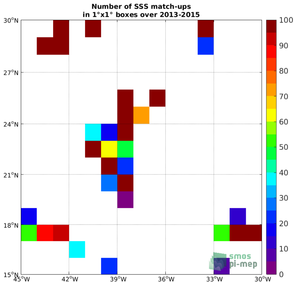
Figure 4: Number of SSS match-ups between TSG (GOSUD-Sailing-ship) SSS and the Aquarius SSS L2 CAP v5 (JPL) SSS product for the SPURS 1 Pi-MEP region over 1°x1° boxes and for the full satellite product period.
