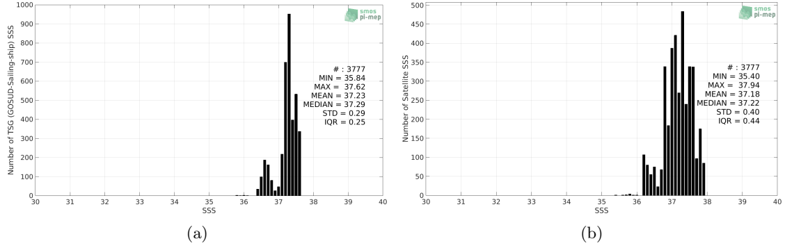
Figure 2: Histograms of SSS from TSG (GOSUD-Sailing-ship) (a) and Aquarius SSS L2 CAP v5 (JPL) (b) considering all match-up pairs per bins of 0.1 over the SPURS 1 Pi-MEP region and for the full satellite product period.
