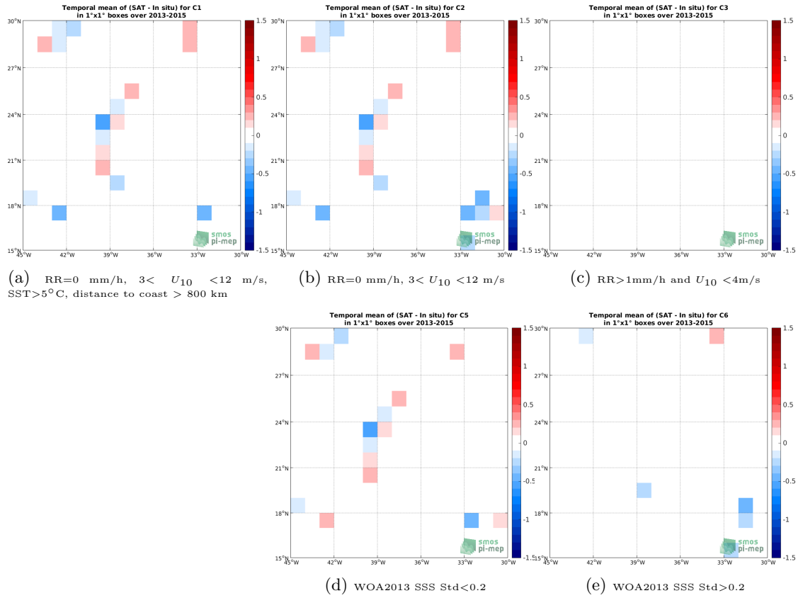
Figure 12: Temporal mean gridded over spatial boxes of size 1^\circ \times 1^\circ of \Delta SSS (Aquarius-L2-JPL-V5 - TSG-GOSUD-Sailing-ship) for 5 different subdatasets corresponding to: RR=0 mm/h, 3 < U_{10} < 12 m/s, SST > 5^\circ C , distance to coast > 800 km (a), RR=0 mm/h, 3 < U_{10} < 12 m/s (b), RR > 1 mm/h and U_{10} < 4 m/s (c), WOA2013 SSS Std < 0.2 (d), WOA2013 SSS Std > 0.2 (e).
