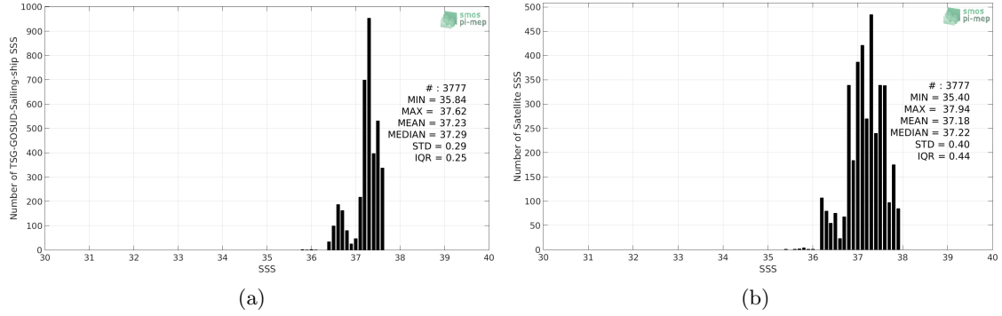
Figure 2: Histograms of SSS from TSG-GOSUD-Sailing-ship (a) and Aquarius-L2-JPL-V5 (b) considering all match-up pairs per bins of 0.1 over the SPURS 1 Pi-MEP region and for the full satellite product period.
