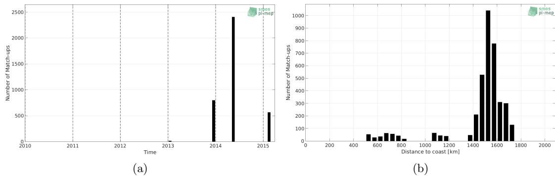
Figure 1: Number of match-ups between TSG-GOSUD-Sailing-ship and Aquarius-L2-JPL-V5 SSS as a function of time (a) and as function of the distance to coast (b) over the SPURS 1 Pi-MEP region and for the full satellite product period.
