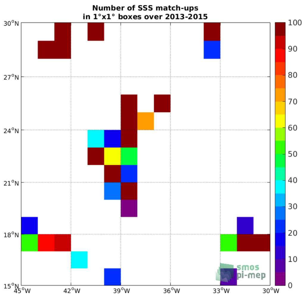
Figure 4: Number of SSS match-ups between TSG-GOSUD-Sailing-ship SSS and the Aquarius-L2-JPL-V5 SSS product for the SPURS 1 Pi-MEP region over 1°x1° boxes and for the full satellite product period.
