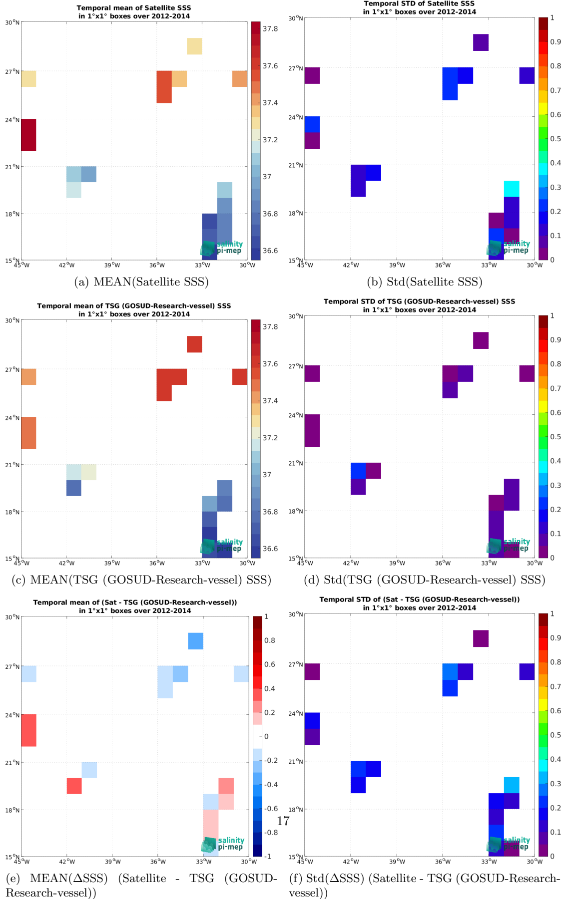
Figure 7: Temporal mean (left) and Std (right) of SSS from Aquarius SSS L2 CAP v5 (JPL) (top), TSG (GOSUD-Research-vessel) (middle), and of \Delta SSS (Satellite - TSG (GOSUD-Research-vessel)). Only match-up pairs are used to generate these maps.
