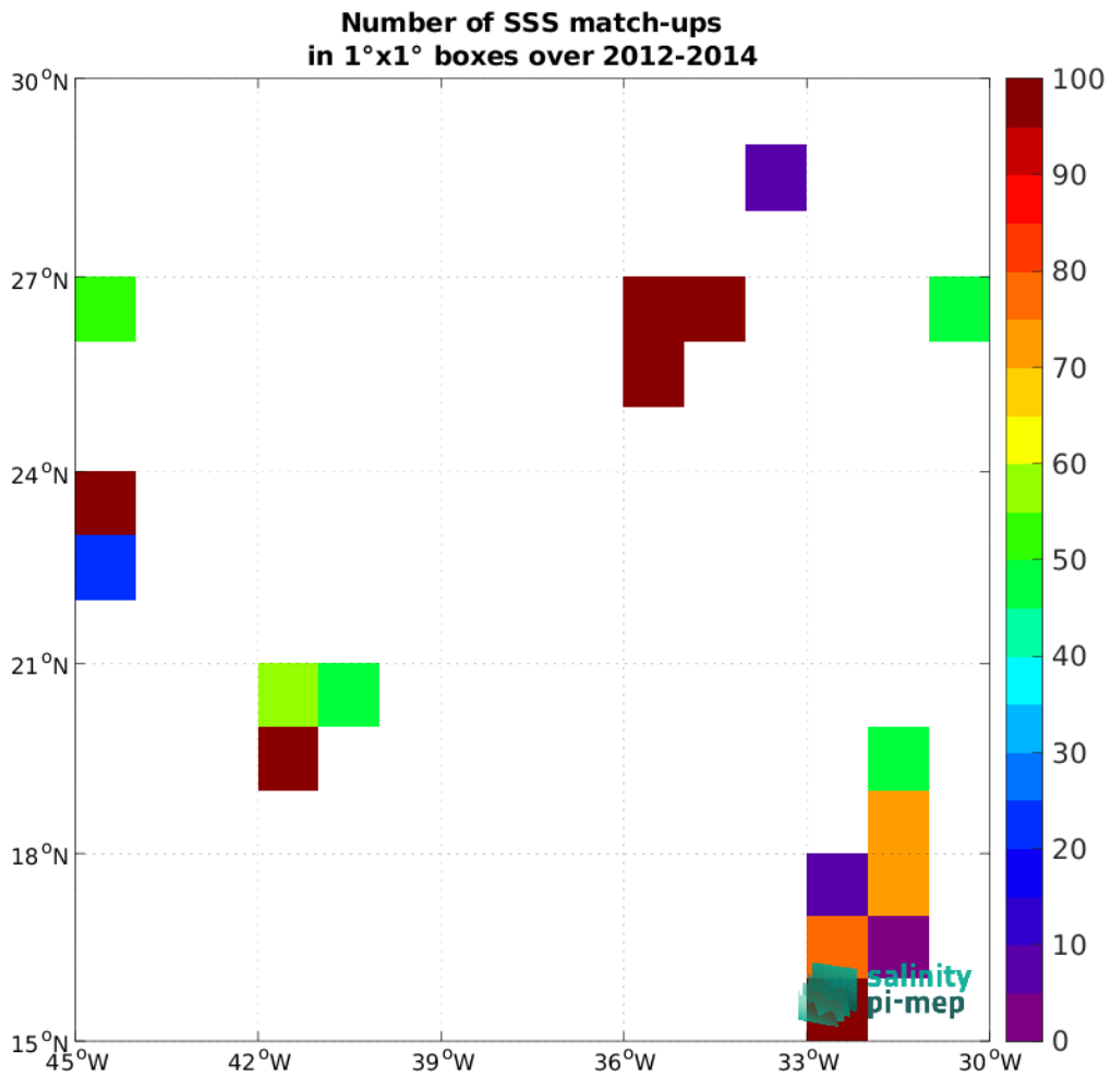
Figure 5: Number of SSS match-ups between TSG (GOSUD-Research-vessel) SSS and the Aquarius SSS L2 CAP v5 (JPL) SSS product for the SPURS 1 Pi-MEP region over 1°x1° boxes and for the full satellite product period.
