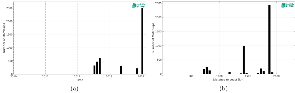
Figure 2: Number of match-ups between TSG (GOSUD-Research-vessel) and Aquarius SSS L2 CAP v5 (JPL) SSS as a function of time (a) and as function of the distance to coast (b) over the SPURS 1 Pi-MEP region and for the full satellite product period.
