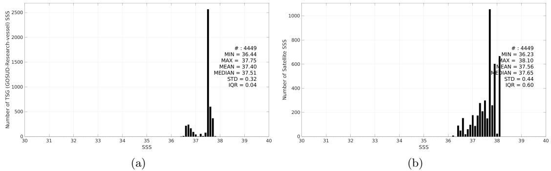
Figure 3: Histograms of SSS from TSG (GOSUD-Research-vessel) (a) and Aquarius SSS L2 CAP v5 (JPL) (b) considering all match-up pairs per bins of 0.1 over the SPURS 1 Pi-MEP region and for the full satellite product period.
