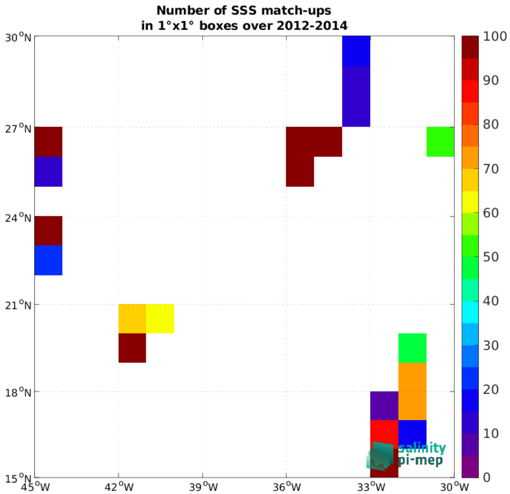
Figure 4: Number of SSS match-ups between TSG (GOSUD-Research-vessel) SSS and the Aquarius SSS L2 CAP v5 (JPL) SSS product for the SPURS 1 Pi-MEP region over 1°×1° boxes and for the full satellite product period.
