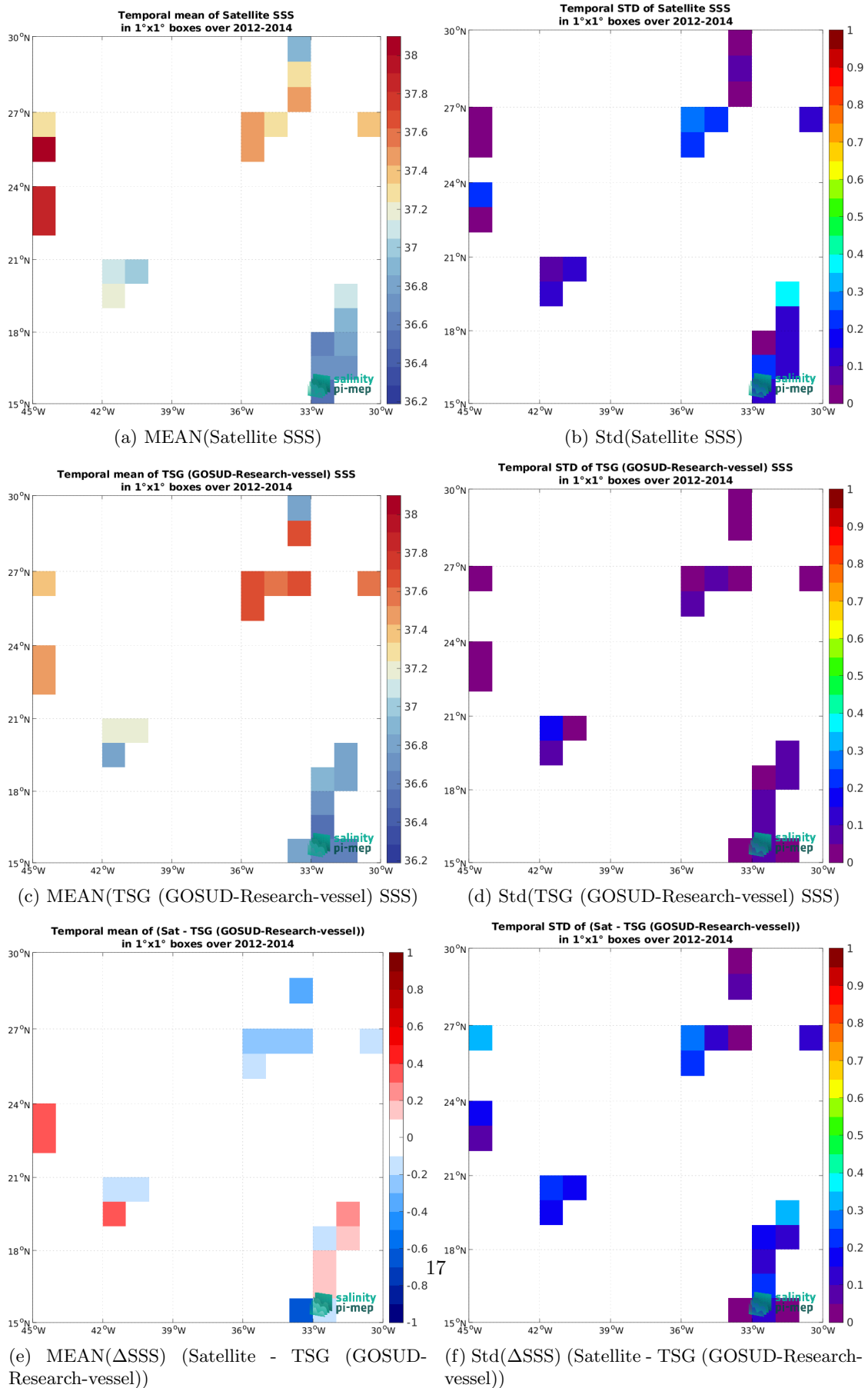
Figure 6: Temporal mean (left) and Std (right) of SSS from Aquarius SSS L2 CAP v5 (JPL) (top), TSG (GOSUD-Research-vessel) (middle), and of \Delta SSS (Satellite - TSG (GOSUD-Research-vessel)). Only match-up pairs are used to generate these maps.
