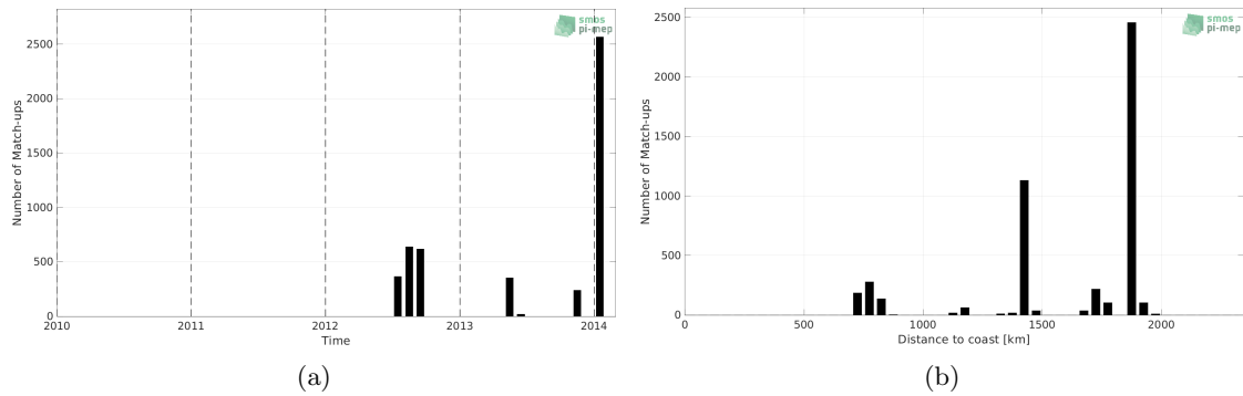
Figure 1: Number of match-ups between TSG (GOSUD-Research-vessel) and Aquarius SSS L2 CAP v5 (JPL) SSS as a function of time (a) and as function of the distance to coast (b) over the SPURS 1 Pi-MEP region and for the full satellite product period.
