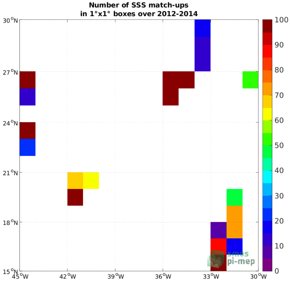
Figure 4: Number of SSS match-ups between TSG (GOSUD-Research-vessel) SSS and the Aquarius SSS L2 CAP v5 (JPL) SSS product for the SPURS 1 Pi-MEP region over 1^\circ \times 1^\circ boxes and for the full satellite product period.
