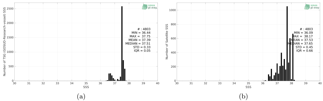
Figure 2: Histograms of SSS from TSG (GOSUD-Research-vessel) (a) and Aquarius SSS L2 CAP v5 (JPL) (b) considering all match-up pairs per bins of 0.1 over the SPURS 1 Pi-MEP region and for the full satellite product period.
