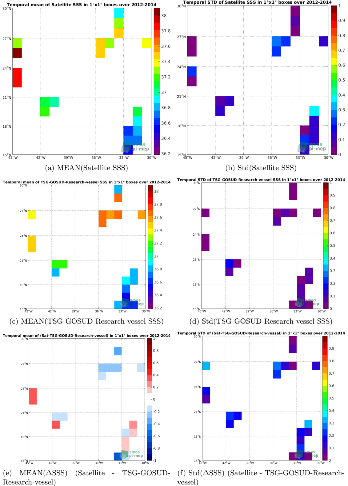
Figure 6: Temporal mean (left) and Std (right) of SSS from Aquarius-L2-JPL-V5 (top), TSG-GOSUD-Research-vessel (middle), and of \Delta SSS (Satellite - TSG-GOSUD-Research-vessel). Only match-up pairs are used to generate these maps.
