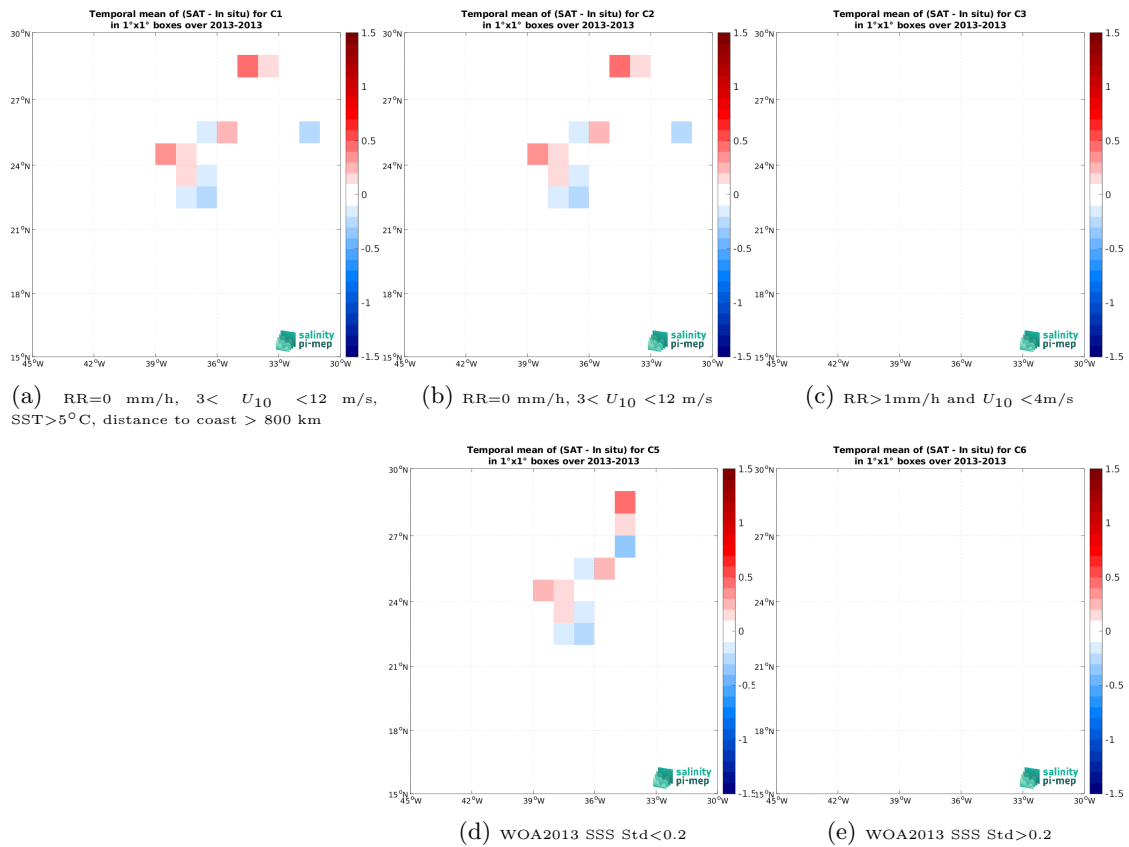
Figure 14: Temporal mean gridded over spatial boxes of size 1^\circ \times 1^\circ of \Delta SSS (Aquarius SSS L2 CAP v5 (JPL) - TSG (CSIC-UTM)) for 5 different subdatasets corresponding to:RR=0 mm/h, 3 < U_{10} < 12 m/s, SST>5°C, distance to coast > 800 km (a), RR=0 mm/h, 3 < U_{10} < 12 m/s (b), RR>1mm/h and U_{10} < 4 m/s (c), WOA2013 SSS Std<0.2 (d), WOA2013 SSS Std>0.2 (e).
