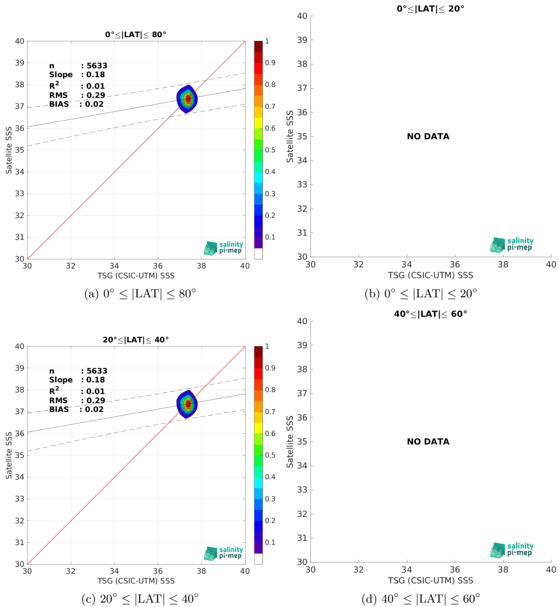
Figure 10: Contour maps of the concentration of Aquarius SSS L2 CAP v5 (JPL) SSS (y-axis) versus TSG (CSIC-UTM) SSS (x-axis) at match-up pairs for different latitude bands. For each plot, the red line shows x=y . The black thin and dashed lines indicate a linear fit through the data cloud and the \pm 95\% confidence levels, respectively. The number match-up pairs n , the slope and R^2 coefficient of the linear fit, the root mean square (RMS) and the mean bias between satellite and in situ data are indicated for each latitude band in each plots.
