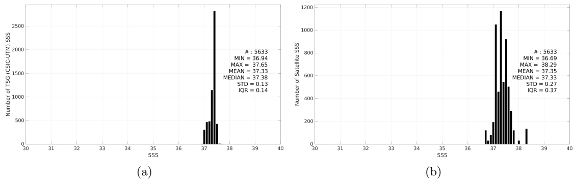
Figure 3: Histograms of SSS from TSG (CSIC-UTM) (a) and Aquarius SSS L2 CAP v5 (JPL) (b) considering all match-up pairs per bins of 0.1 over the SPURS 1 Pi-MEP region and for the full satellite product period.
