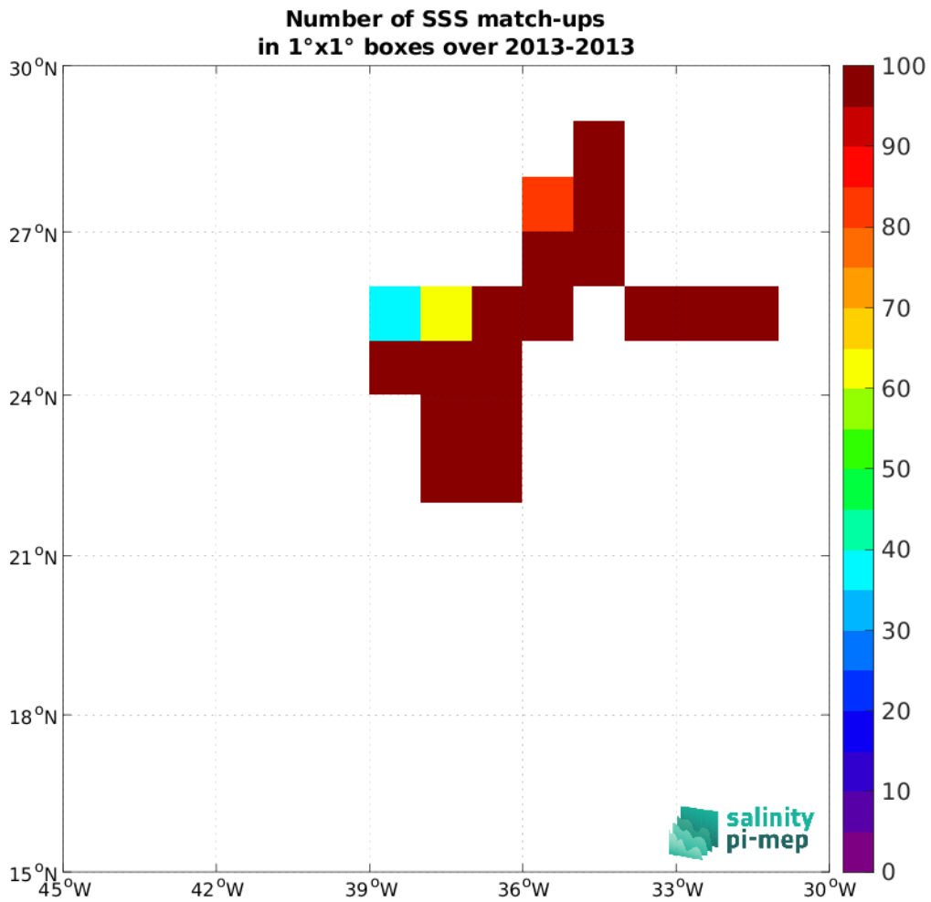
Figure 5: Number of SSS match-ups between TSG (CSIC-UTM) SSS and the Aquarius SSS L2 CAP v5 (JPL) SSS product for the SPURS 1 Pi-MEP region over 1^\circ \times 1^\circ boxes and for the full satellite product period.
