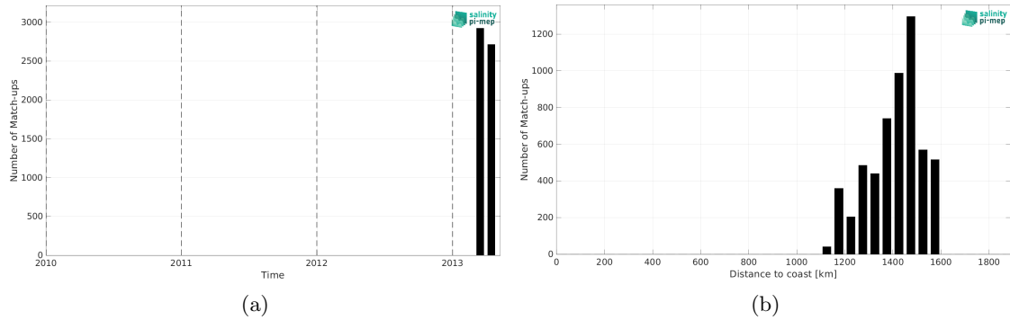
Figure 2: Number of match-ups between TSG (CSIC-UTM) and Aquarius SSS L2 CAP v5 (JPL) SSS as a function of time (a) and as function of the distance to coast (b) over the SPURS 1 Pi-MEP region and for the full satellite product period.
