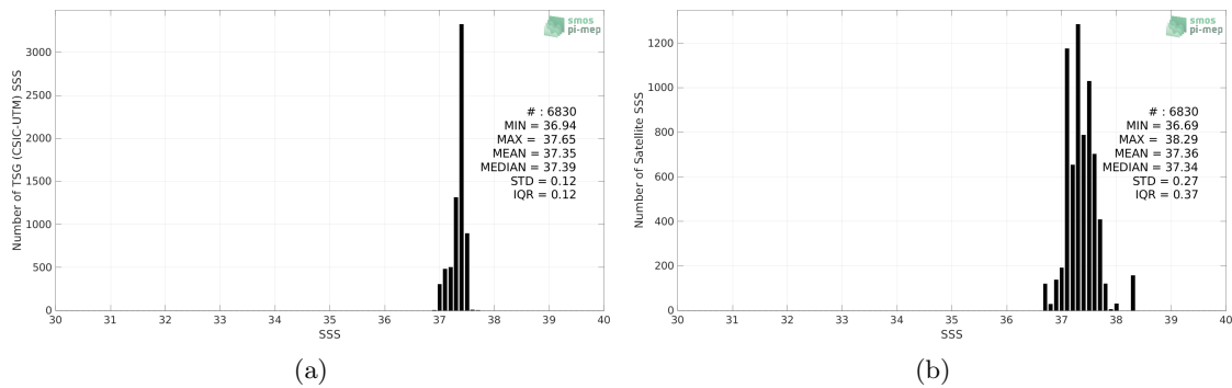
Figure 2: Histograms of SSS from TSG (CSIC-UTM) (a) and Aquarius SSS L2 CAP v5 (JPL) (b) considering all match-up pairs per bins of 0.1 over the SPURS 1 Pi-MEP region and for the full satellite product period.
