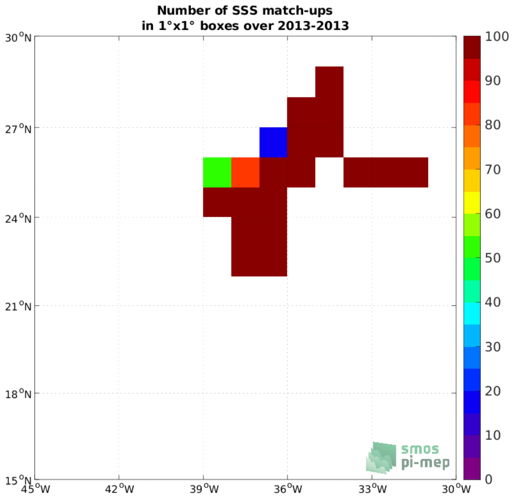
Figure 4: Number of SSS match-ups between TSG (CSIC-UTM) SSS and the Aquarius SSS L2 CAP v5 (JPL) SSS product for the SPURS 1 Pi-MEP region over 1^\circ \times 1^\circ boxes and for the full satellite product period.
