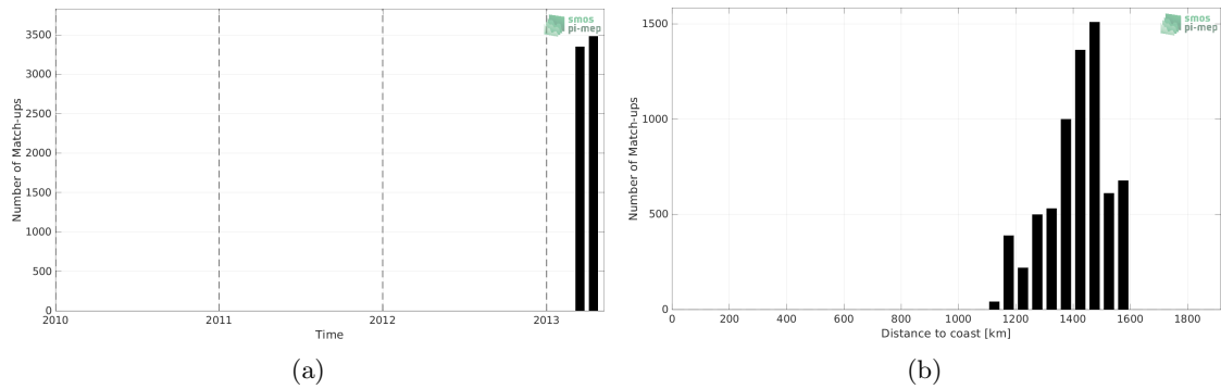
Figure 1: Number of match-ups between TSG (CSIC-UTM) and Aquarius SSS L2 CAP v5 (JPL) SSS as a function of time (a) and as function of the distance to coast (b) over the SPURS 1 Pi-MEP region and for the full satellite product period.
