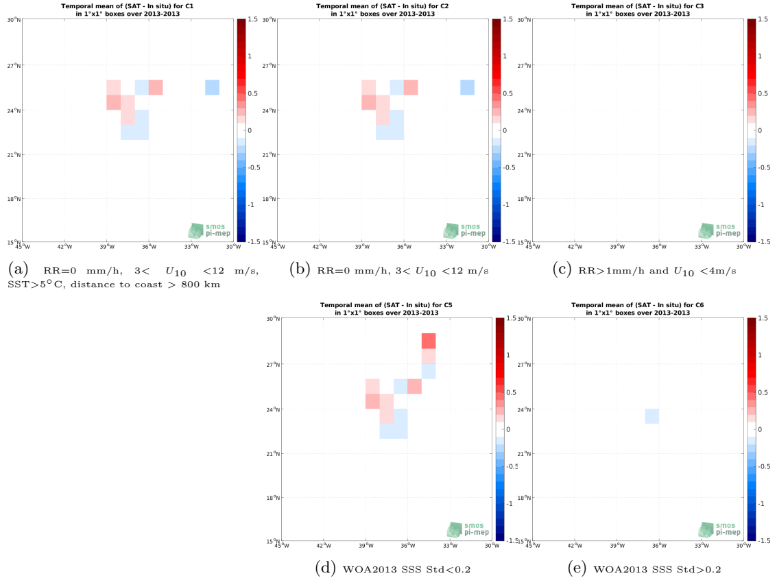
Figure 12: Temporal mean gridded over spatial boxes of size 1^{\circ}\times 1^{\circ} of \Delta\text{SSS} (Aquarius SSS L2 CAP v5 (JPL) - TSG (CSIC-UTM)) for 5 different subdatasets corresponding to:RR=0 mm/h, 3 < U_{10} < 12 m/s, SST >5^{\circ}\text{C} , distance to coast > 800 km (a), RR=0 mm/h, 3 < U_{10} < 12 m/s (b), RR >1 mm/h and U_{10} < 4 m/s (c), WOA2013 SSS Std <0.2 (d), WOA2013 SSS Std >0.2 (e).
