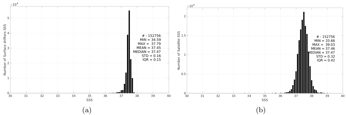
Figure 3: Histograms of SSS from Surface drifters (a) and Aquarius SSS L2 CAP v5 (JPL) (b) considering all match-up pairs per bins of 0.1 over the SPURS 1 Pi-MEP region and for the full satellite product period.
