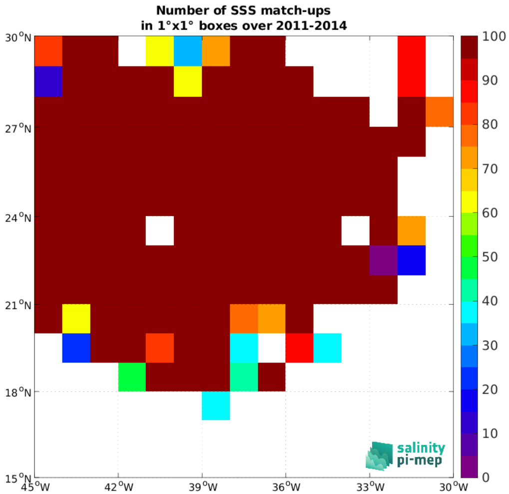
Figure 4: Number of SSS match-ups between Surface drifters SSS and the Aquarius SSS L2 CAP v5 (JPL) SSS product for the SPURS 1 Pi-MEP region over 1°×1° boxes and for the full satellite product period.
