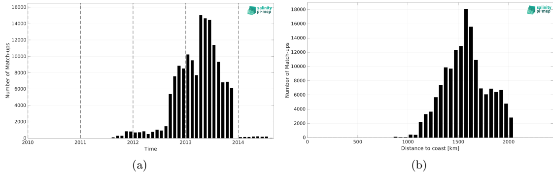
Figure 2: Number of match-ups between Surface drifters and Aquarius SSS L2 CAP v5 (JPL) SSS as a function of time (a) and as function of the distance to coast (b) over the SPURS 1 Pi-MEP region and for the full satellite product period.
