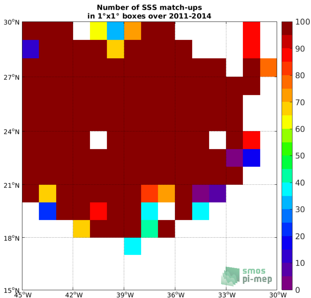
Figure 3: Number of SSS match-ups between Surface drifters SSS and the Aquarius SSS L2 CAP v5 (JPL) SSS product for the SPURS 1 Pi-MEP region over 1°x1° boxes and for the full satellite product period.
