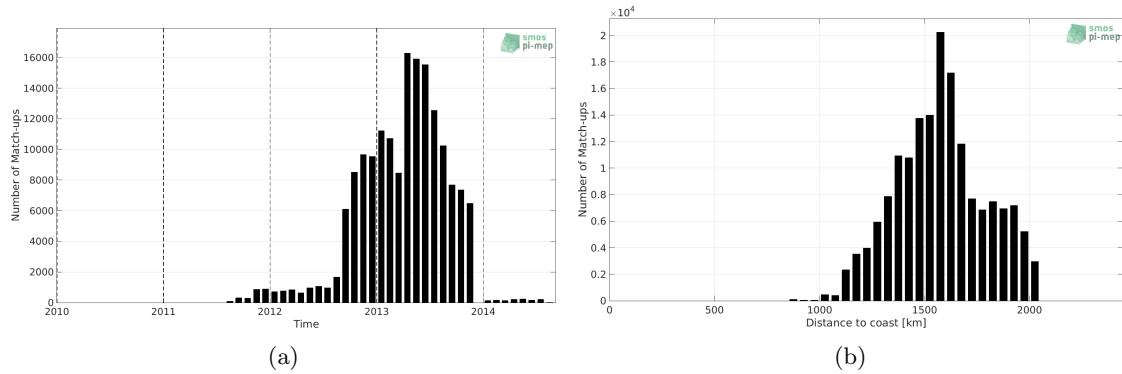
Figure 1: Number of match-ups between Surface drifters and Aquarius SSS L2 CAP v5 (JPL) SSS as a function of time (a) and as function of the distance to coast (b) over the SPURS 1 Pi-MEP region and for the full satellite product period.
