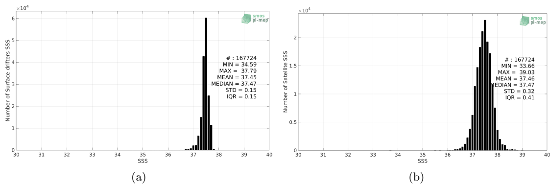
Figure 2: Histograms of SSS from Surface drifters (a) and Aquarius SSS L2 CAP v5 (JPL) (b) considering all match-up pairs per bins of 0.1 over the SPURS 1 Pi-MEP region and for the full satellite product period.
