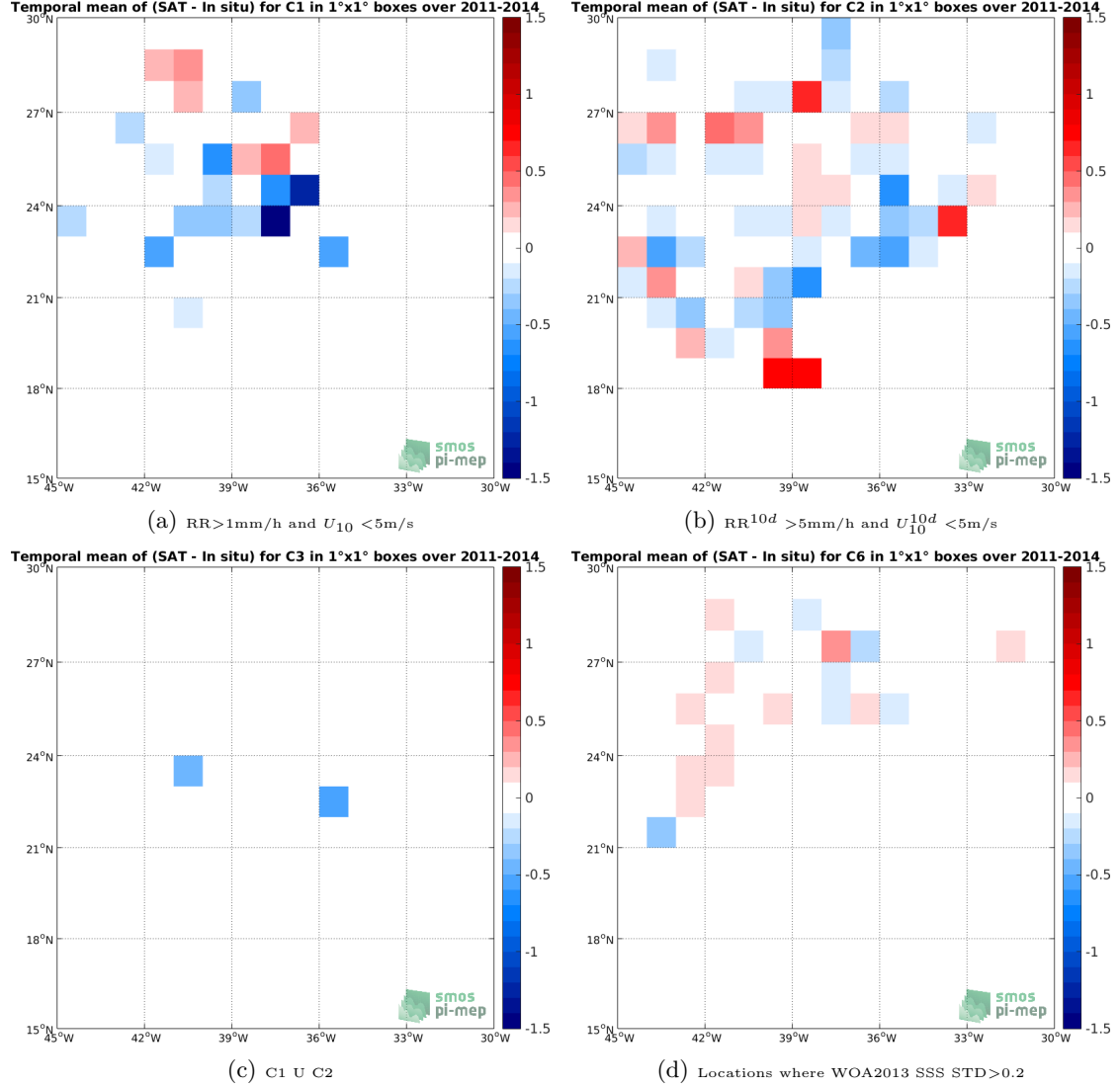
Figure 11: Temporal mean gridded over spatial boxes of size 1^\circ \times 1^\circ of \Delta SSS (Aquarius-L2-JPL-V5 - Surface drifters) for 4 different subdatasets corresponding to: RR > 1 \text{ mm/h} and U_{10} < 5 \text{ m/s} (a), RR^{10d} > 5 \text{ mm/h} and U_{10}^{10d} < 5 \text{ m/s} (b), C1 U C2 (c), Locations where WOA2013 SSS STD > 0.2 (d).
