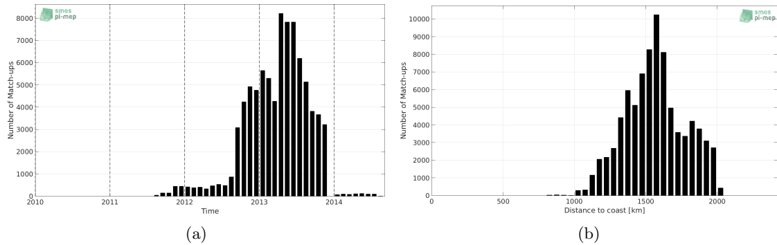
Figure 1: Number of match-ups between Surface drifters and Aquarius-L2-JPL-V5 SSS as a function of time (a) and as function of the distance to coast (b) over the SPURS 1 Pi-MEP region and for the full satellite product period.
