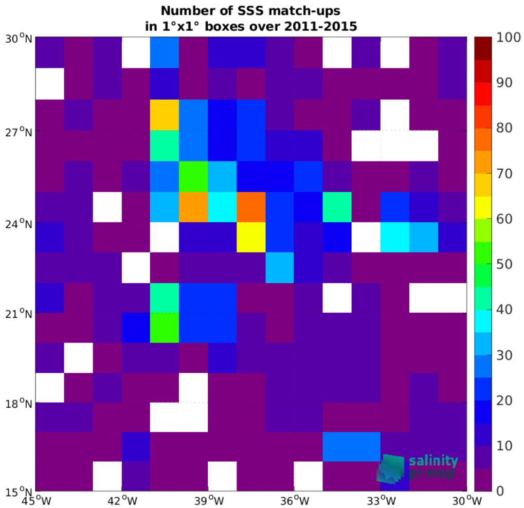
Figure 5: Number of SSS match-ups between Argo SSS and the Aquarius SSS L2 CAP v5 (JPL) SSS product for the SPURS 1 Pi-MEP region over 1^\circ \times 1^\circ boxes and for the full satellite product period.
