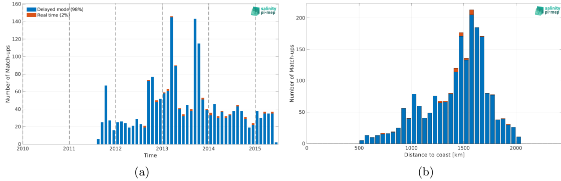
Figure 2: Number of match-ups between Argo and Aquarius SSS L2 CAP v5 (JPL) SSS as a function of time (a) and as function of the distance to coast (b) over the SPURS 1 Pi-MEP region and for the full satellite product period.
