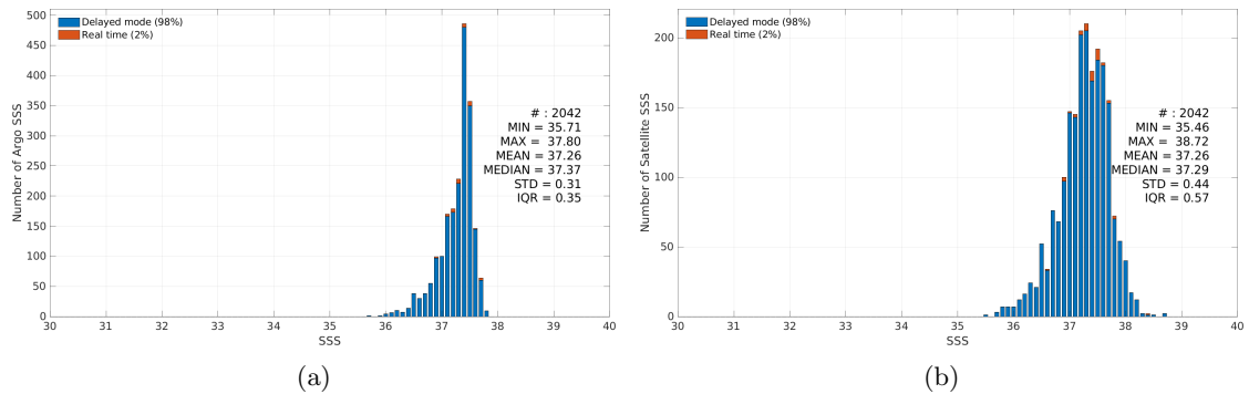
Figure 3: Histograms of SSS from Argo (a) and Aquarius SSS L2 CAP v5 (JPL) (b) considering all match-up pairs per bins of 0.1 over the SPURS 1 Pi-MEP region and for the full satellite product period.
