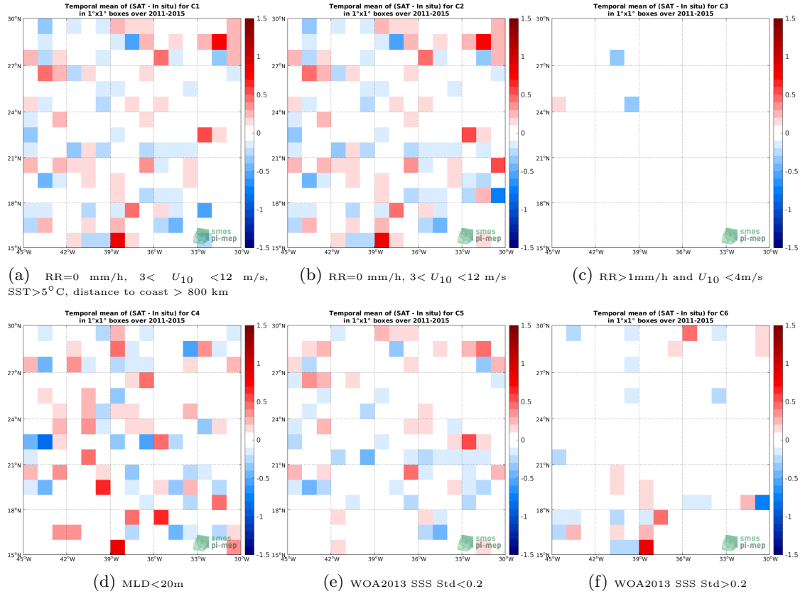
Figure 12: Temporal mean gridded over spatial boxes of size 1^\circ \times 1^\circ of \Delta SSS (Aquarius SSS L2 CAP v5 (JPL) - Argo) for 6 different subdatasets corresponding to:RR=0 mm/h, 3 < U_{10} < 12 m/s, SST>5°C, distance to coast > 800 km (a), RR=0 mm/h, 3 < U_{10} < 12 m/s (b), RR>1mm/h and U_{10} < 4 m/s (c),MLD<20m (d),WOA2013 SSS Std<0.2 (e),WOA2013 SSS Std>0.2 (f).
