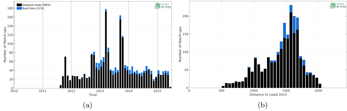
Figure 1: Number of match-ups between Argo and Aquarius SSS L2 CAP v5 (JPL) SSS as a function of time (a) and as function of the distance to coast (b) over the SPURS 1 Pi-MEP region and for the full satellite product period.
