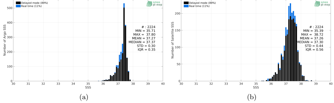
Figure 2: Histograms of SSS from Argo (a) and Aquarius SSS L2 CAP v5 (JPL) (b) considering all match-up pairs per bins of 0.1 over the SPURS 1 Pi-MEP region and for the full satellite product period.
