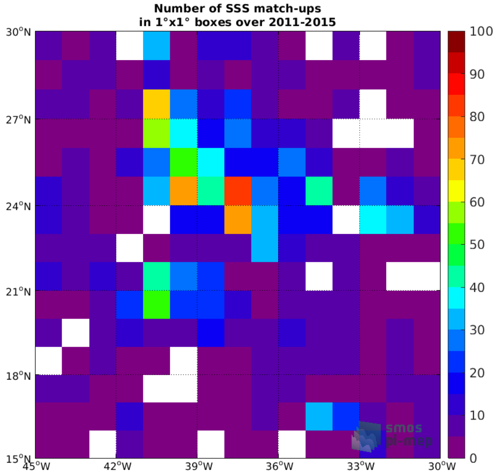
Figure 4: Number of SSS match-ups between Argo SSS and the Aquarius SSS L2 CAP v5 (JPL) SSS product for the SPURS 1 Pi-MEP region over 1°x1° boxes and for the full satellite product period.
