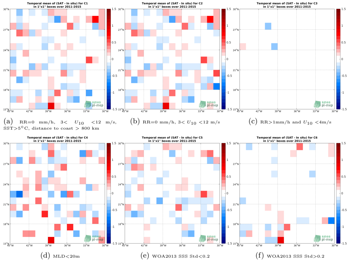
Figure 12: Temporal mean gridded over spatial boxes of size 1^\circ \times 1^\circ of \Delta SSS (Aquarius-L2-JPL-V5 - Argo) for 6 different subdatasets corresponding to: RR=0 mm/h, 3 < U_{10} < 12 m/s, SST > 5^\circ C , distance to coast > 800 km (a), RR=0 mm/h, 3 < U_{10} < 12 m/s (b), RR > 1 mm/h and U_{10} < 4 m/s (c), MLD < 20 m (d), WOA2013 SSS Std < 0.2 (e), WOA2013 SSS Std > 0.2 (f).
