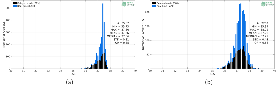
Figure 2: Histograms of SSS from Argo (a) and Aquarius-L2-JPL-V5 (b) considering all match-up pairs per bins of 0.1 over the SPURS 1 Pi-MEP region and for the full satellite product period.
