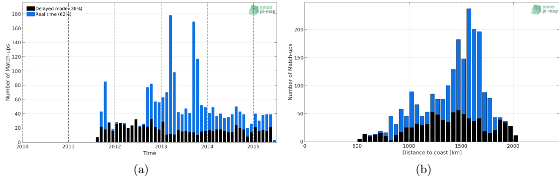
Figure 1: Number of match-ups between Argo and Aquarius-L2-JPL-V5 SSS as a function of time (a) and as function of the distance to coast (b) over the SPURS 1 Pi-MEP region and for the full satellite product period.
