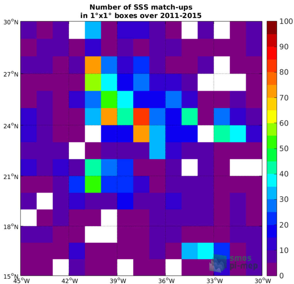
Figure 4: Number of SSS match-ups between Argo SSS and the Aquarius-L2-JPL-V5 SSS product for the SPURS 1 Pi-MEP region over 1°x1° boxes and for the full satellite product period.
