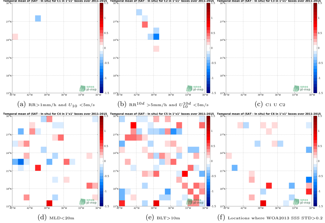
Figure 12: Temporal mean gridded over spatial boxes of size 1^\circ \times 1^\circ of \Delta\text{SSS} (Aquarius-L2-JPL-V5 - Argo) for 6 different subdatasets corresponding to: \text{RR} > 1\text{mm/h} and U_{10} < 5\text{m/s} (a), \text{RR}^{10d} > 5\text{mm/h} and U_{10}^{10d} < 5\text{m/s} (b), C1 U C2 (c), \text{MLD} < 20\text{m} (d), \text{BLT} > 10\text{m} (e), Locations where WOA2013 SSS STD > 0.2 (f).
