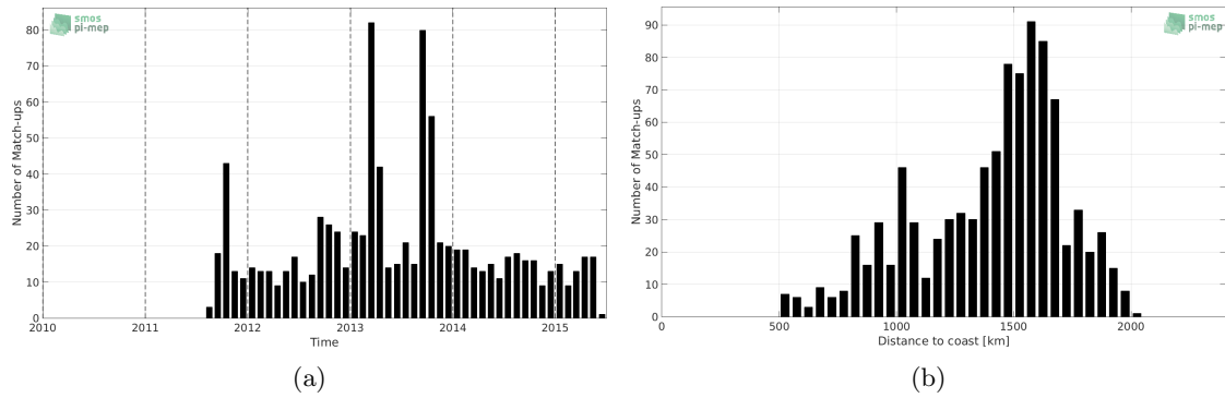
Figure 1: Number of match-ups between Argo and Aquarius-L2-JPL-V5 SSS as a function of time (a) and as function of the distance to coast (b) over the SPURS 1 Pi-MEP region and for the full satellite product period.
