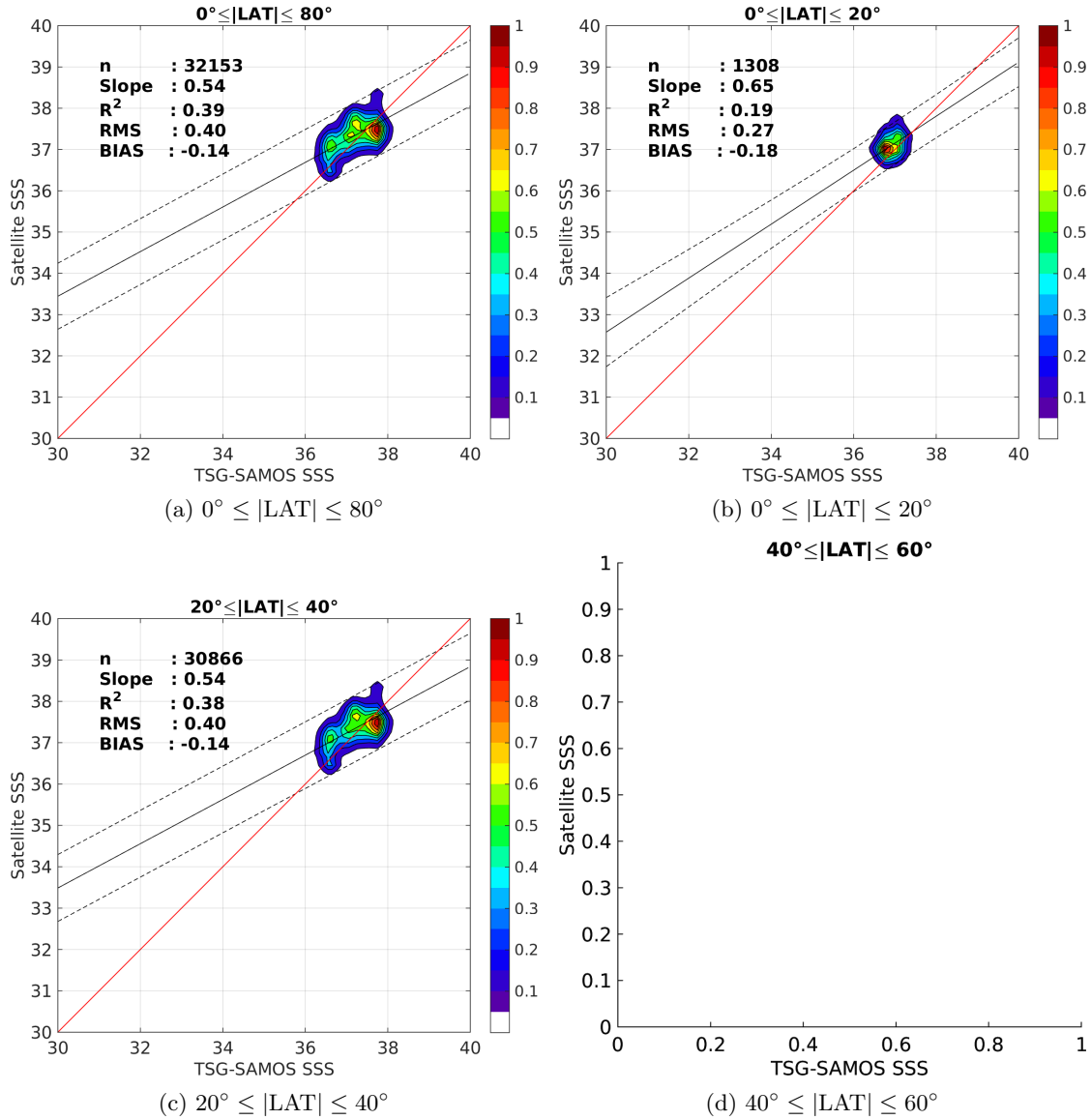
Figure 9: Contour maps of the concentration of AQUARIUS-L2-JPL-V4 SSS (y-axis) versus TSG-SAMOS SSS (x-axis) at match-up pairs for different latitude bands. For each plot, the red line shows x=y . The black thin and dashed lines indicate a linear fit through the data cloud and the \pm 95\% confidence levels, respectively. The number match-up pairs n , the slope and R^2 coefficient of the linear fit, the root mean square (RMS) and the mean bias between satellite and in situ data are indicated for each latitude band in each plots.
