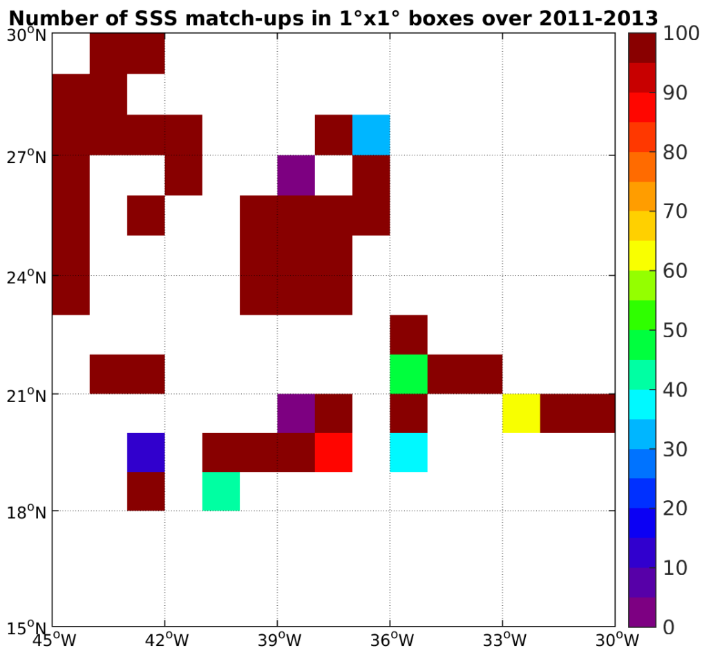
Figure 4: Number of SSS match-ups between TSG-SAMOS SSS and the AQUARIUS-L2-JPL-V4 SSS product for the SPURS 1 Pi-MEP region over 1°x1° boxes and for the full satellite product period.
