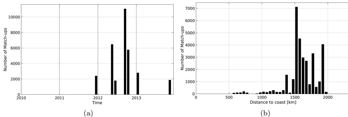
Figure 1: Number of match-ups between TSG-SAMOS and AQUARIUS-L2-JPL-V4 SSS as a function of time (a) and as function of the distance to coast (b) over the SPURS 1 Pi-MEP region and for the full satellite product period.
