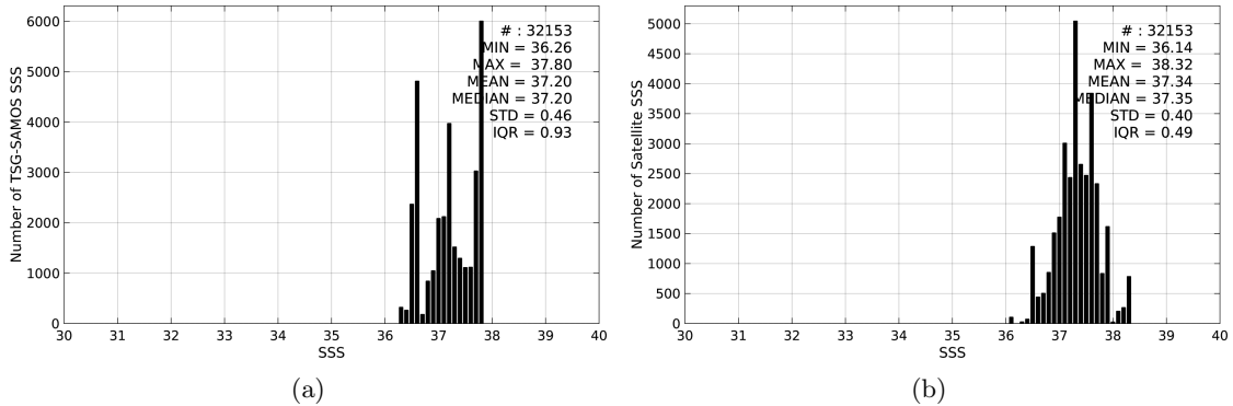
Figure 2: Histograms of SSS from TSG-SAMOS (a) and AQUARIUS-L2-JPL-V4 (b) considering all match-up pairs per bins of 0.1 over the SPURS 1 Pi-MEP region and for the full satellite product period.
