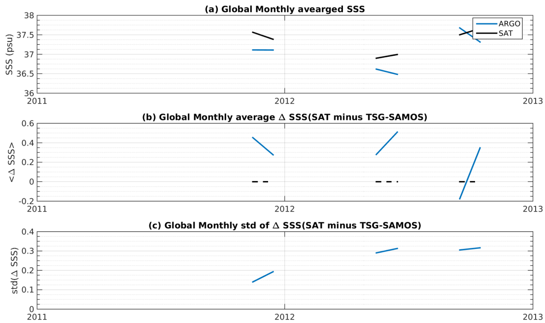
Figure 7: Time series of the monthly averaged mean SSS (top), mean \Delta SSS (Satellite - TSG-SAMOS) and STD of \Delta SSS (Satellite - TSG-SAMOS) over the SPURS 1 Pi-MEP region considering all match-ups collected by the Pi-MEP platform.
