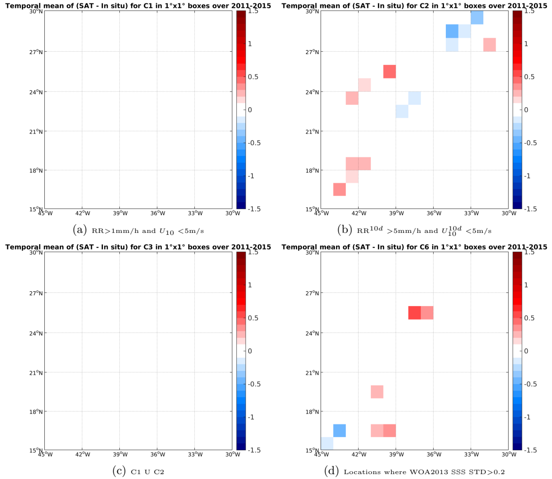
Figure 12: Temporal mean gridded over spatial boxes of size 1^\circ \times 1^\circ of \Delta SSS (AQUARIUS-L2-JPL-V4 - TSG-LEGOS-DM) for 4 different subdatasets corresponding to: RR > 1 mm/h and U_{10} < 5 m/s (a), RR 10d > 5 mm/h and U_{10}^{10d} < 5 m/s (b), C1 U C2 (c), Locations where WOA2013 SSS STD > 0.2 (d).
