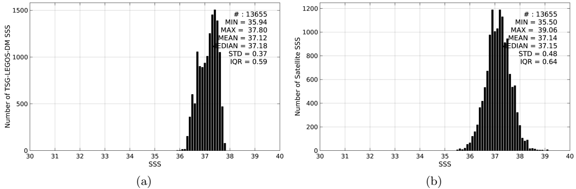
Figure 2: Histograms of SSS from TSG-LEGOS-DM (a) and AQUARIUS-L2-JPL-V4 (b) considering all match-up pairs per bins of 0.1 over the SPURS 1 Pi-MEP region and for the full satellite product period.
