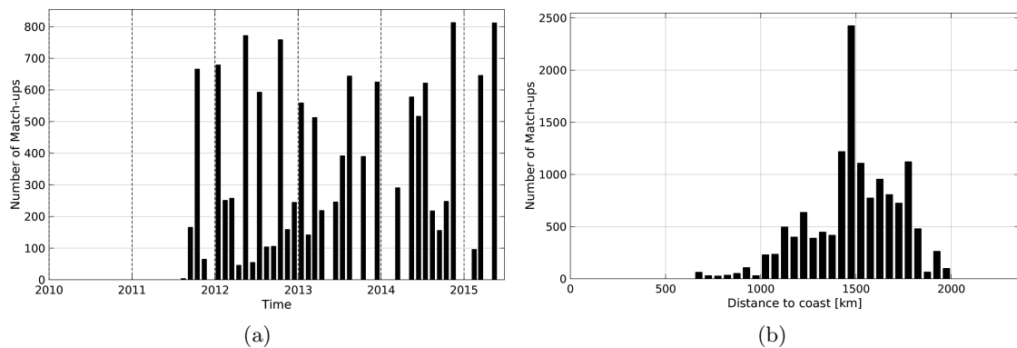
Figure 1: Number of match-ups between TSG-LEGOS-DM and AQUARIUS-L2-JPL-V4 SSS as a function of time (a) and as function of the distance to coast (b) over the SPURS 1 Pi-MEP region and for the full satellite product period.
