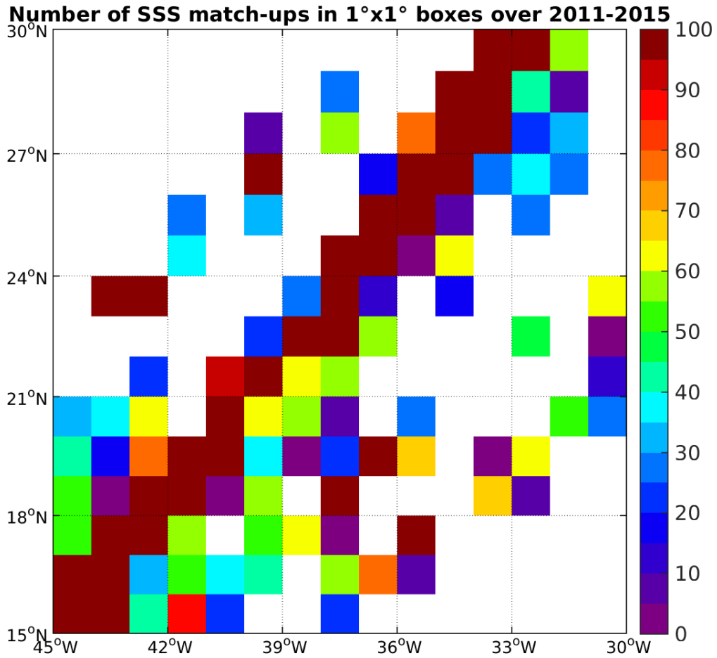
Figure 4: Number of SSS match-ups between TSG-LEGOS-DM SSS and the AQUARIUS-L2-JPL-V4 SSS product for the SPURS 1 Pi-MEP region over 1°x1° boxes and for the full satellite product period.
