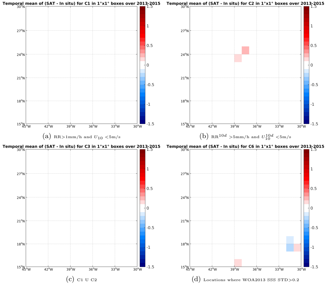
Figure 12: Temporal mean gridded over spatial boxes of size 1°x1° of \Delta SSS (AQUARIUS-L2-JPL-V4 - TSG-GOSUD-Sailing-ship) for 4 different subdatasets corresponding to:RR>1mm/h and U_{10} < 5\text{m/s} (a), RR^{10d} > 5\text{mm/h} and U_{10}^{10d} < 5\text{m/s} (b), C1 U C2 (c),Locations where WOA2013 SSS STD>0.2 (d).
