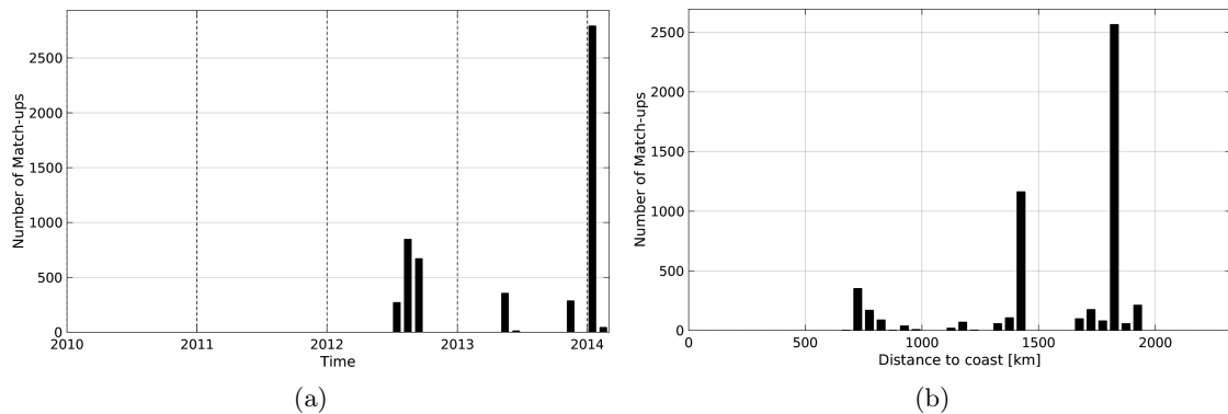
Figure 1: Number of match-ups between TSG-GOSUD-Research-vessel and AQUARIUS-L2-JPL-V4 SSS as a function of time (a) and as function of the distance to coast (b) over the SPURS 1 Pi-MEP region and for the full satellite product period.
