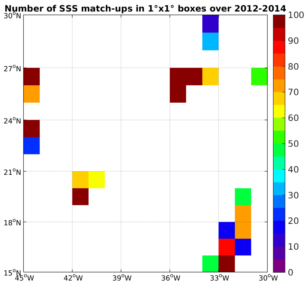
Figure 4: Number of SSS match-ups between TSG-GOSUD-Research-vessel SSS and the AQUARIUS-L2-JPL-V4 SSS product for the SPURS 1 Pi-MEP region over 1°x1° boxes and for the full satellite product period.
