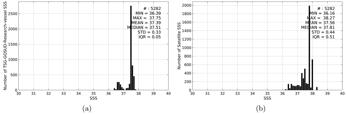
Figure 2: Histograms of SSS from TSG-GOSUD-Research-vessel (a) and AQUARIUS-L2-JPL-V4 (b) considering all match-up pairs per bins of 0.1 over the SPURS 1 Pi-MEP region and for the full satellite product period.
