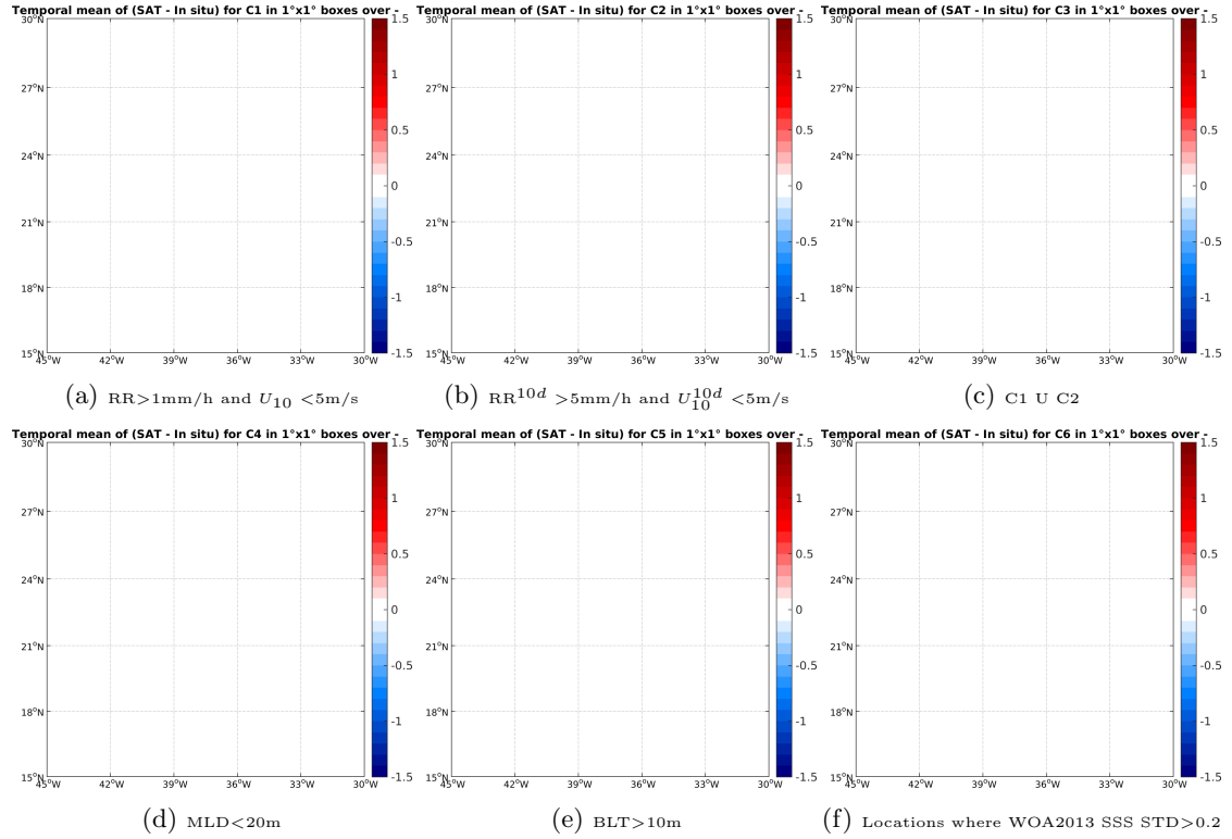
Figure 12: Temporal mean gridded over spatial boxes of size 1^\circ \times 1^\circ of \Delta SSS (AQUARIUS-L2-JPL-V4 - Sea mammals) for 6 different subdatasets corresponding to: RR > 1\text{mm/h} and U_{10} < 5\text{m/s} (a), RR^{10d} > 5\text{mm/h} and U_{10}^{10d} < 5\text{m/s} (b), C1 U C2 (c), MLD < 20\text{m} (d), BLT > 10\text{m} (e), Locations where WOA2013 SSS STD > 0.2 (f).
