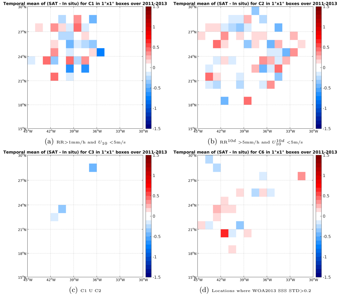
Figure 11: Temporal mean gridded over spatial boxes of size 1^\circ \times 1^\circ of \Delta SSS (AQUARIUS-L2-JPL-V4 - Surface drifters) for 4 different subdatasets corresponding to: RR > 1\text{mm/h} and U_{10} < 5\text{m/s} (a), RR^{10d} > 5\text{mm/h} and U_{10}^{10d} < 5\text{m/s} (b), C1 U C2 (c), Locations where WOA2013 SSS STD > 0.2 (d).
