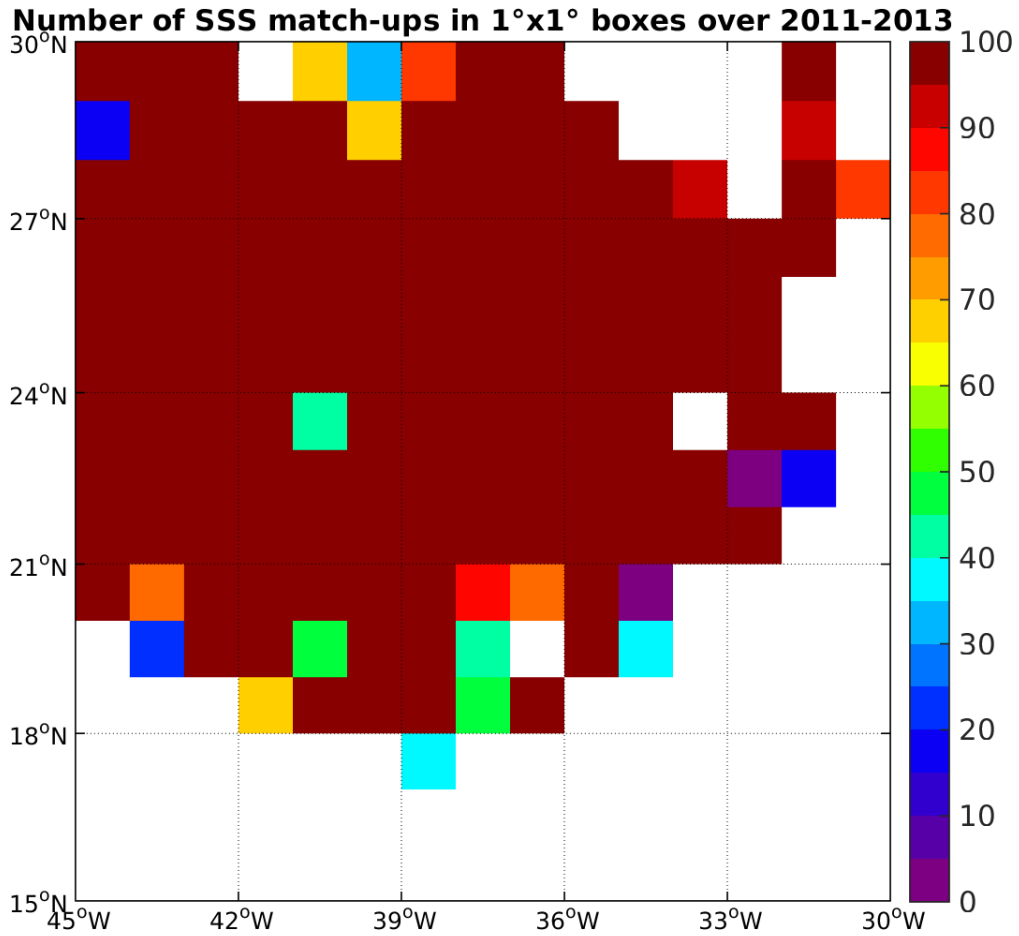
Figure 3: Number of SSS match-ups between Surface drifters SSS and the AQUARIUS-L2-JPL-V4 SSS product for the SPURS 1 Pi-MEP region over 1°x1° boxes and for the full satellite product period.
