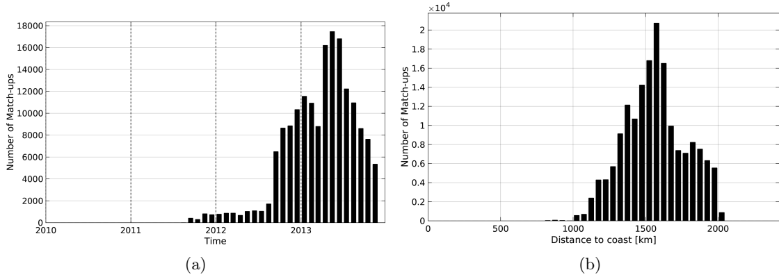
Figure 1: Number of match-ups between Surface drifters and AQUARIUS-L2-JPL-V4 SSS as a function of time (a) and as function of the distance to coast (b) over the SPURS 1 Pi-MEP region and for the full satellite product period.
