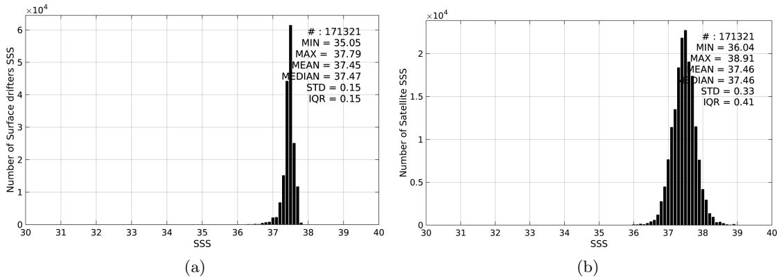
Figure 2: Histograms of SSS from Surface drifters (a) and AQUARIUS-L2-JPL-V4 (b) considering all match-up pairs per bins of 0.1 over the SPURS 1 Pi-MEP region and for the full satellite product period.
