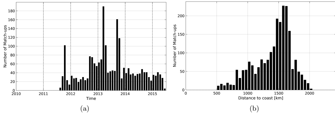
Figure 1: Number of match-ups between Argo and AQUARIUS-L2-JPL-V4 SSS as a function of time (a) and as function of the distance to coast (b) over the SPURS 1 Pi-MEP region and for the full satellite product period.
