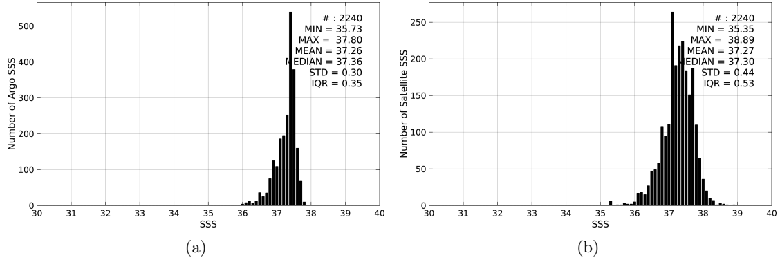
Figure 2: Histograms of SSS from Argos (a) and AQUARIUS-L2-JPL-V4 (b) considering all match-up pairs per bins of 0.1 over the SPURS 1 Pi-MEP region and for the full satellite product period.
