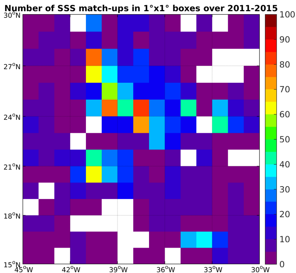
Figure 4: Number of SSS match-ups between Argo SSS and the AQUARIUS-L2-JPL-V4 SSS product for the SPURS 1 Pi-MEP region over 1°x1° boxes and for the full satellite product period.
