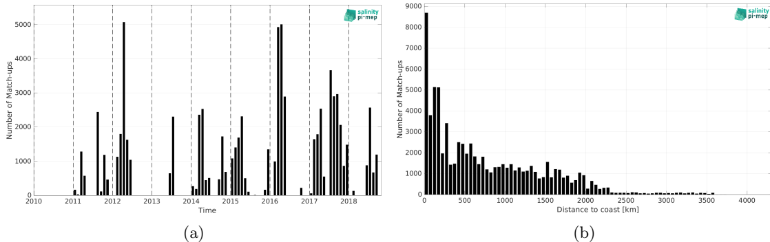
Figure 1: Number of match-ups between TSG (SAMOS) and SMOS and SMAP SSS L4 OI v1 - 7 Days (LOPS) SSS as a function of time (a) and as function of the distance to coast (b) over the South Pacific Ocean Pi-MEP region and for the full satellite product period.
