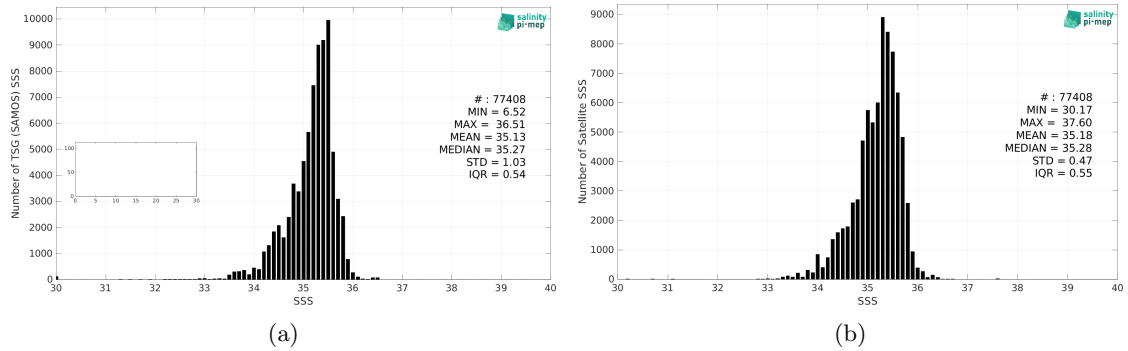
Figure 2: Histograms of SSS from TSG (SAMOS) (a) and SMOS and SMAP SSS L4 OI v1 - 7 Days (LOPS) (b) considering all match-up pairs per bins of 0.1 over the South Pacific Ocean Pi-MEP region and for the full satellite product period.
