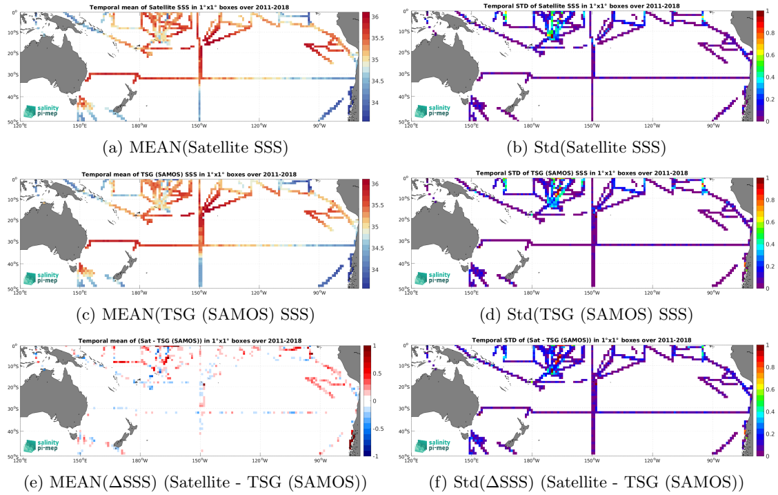
Figure 6: Temporal mean (left) and Std (right) of SSS from SMOS and SMAP SSS L4 OI v1 - 7 Days (LOPS) (top), TSG (SAMOS) (middle), and of \Delta SSS (Satellite - TSG (SAMOS)). Only match-up pairs are used to generate these maps.
