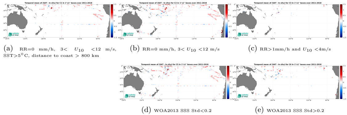
Figure 12: Temporal mean gridded over spatial boxes of size 1^\circ \times 1^\circ of \Delta\text{SSS} (SMOS and SMAP SSS L4 OI v1 - 7 Days (LOPS) - TSG (SAMOS)) for 5 different subdatasets corresponding to:RR=0 mm/h, 3 < U_{10} < 12 m/s, SST >5^\circ\text{C} , distance to coast > 800 km (a), RR=0 mm/h, 3 < U_{10} < 12 m/s (b), RR >1 mm/h and U_{10} < 4 m/s (c), WOA2013 SSS Std <0.2 (d), WOA2013 SSS Std >0.2 (e).
