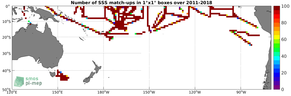
Figure 4: Number of SSS match-ups between TSG (SAMOS) SSS and the SMOS and SMAP SSS L4 OI v1 - 7 Days (LOPS) SSS product for the South Pacific Ocean Pi-MEP region over 1^\circ \times 1^\circ boxes and for the full satellite product period.
