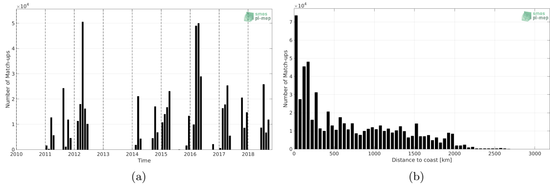
Figure 1: Number of match-ups between TSG (SAMOS) and SMOS and SMAP SSS L4 OI v1 - 7 Days (LOPS) SSS as a function of time (a) and as function of the distance to coast (b) over the South Pacific Ocean Pi-MEP region and for the full satellite product period.
