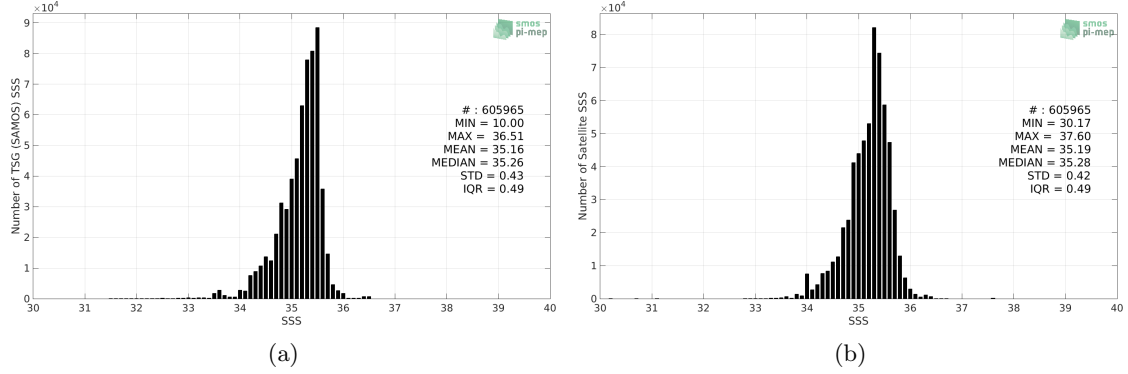
Figure 2: Histograms of SSS from TSG (SAMOS) (a) and SMOS and SMAP SSS L4 OI v1 - 7 Days (LOPS) (b) considering all match-up pairs per bins of 0.1 over the South Pacific Ocean Pi-MEP region and for the full satellite product period.
