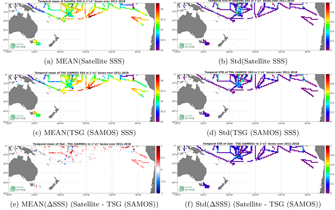
Figure 6: Temporal mean (left) and Std (right) of SSS from SMOS and SMAP SSS L4 OI v1 - 7 Days (LOPS) (top), TSG (SAMOS) (middle), and of \Delta\text{SSS} (Satellite - TSG (SAMOS)). Only match-up pairs are used to generate these maps.
