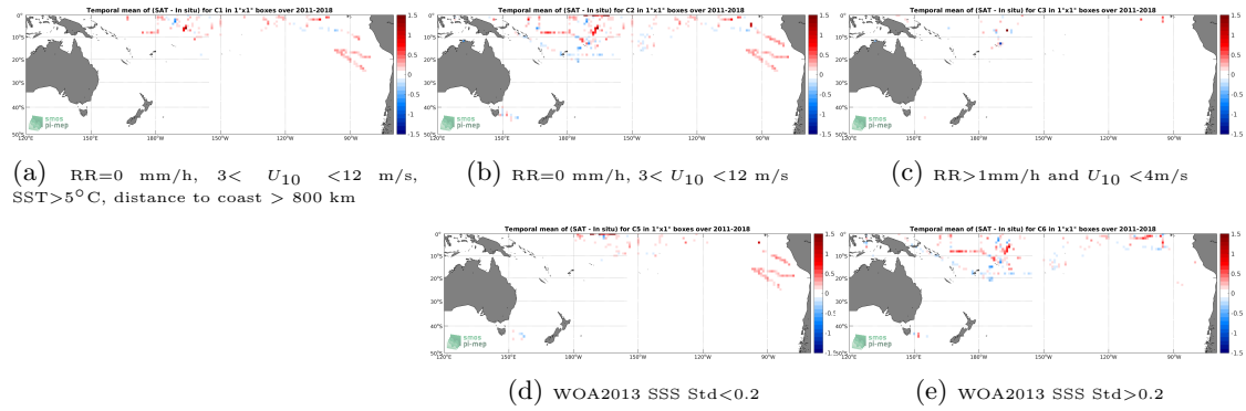
Figure 12: Temporal mean gridded over spatial boxes of size 1^\circ \times 1^\circ of \Delta SSS (SMOS and SMAP SSS L4 OI v1 - 7 Days (LOPS) - TSG (SAMOS)) for 5 different subdatasets corresponding to: RR=0 mm/h, 3 < U_{10} < 12 m/s, SST >5^\circ\text{C} , distance to coast > 800 km (a), RR=0 mm/h, 3 < U_{10} < 12 m/s (b), RR>1\text{mm/h} and U_{10} < 4\text{m/s} (c), WOA2013 SSS Std <0.2 (d), WOA2013 SSS Std >0.2 (e).
