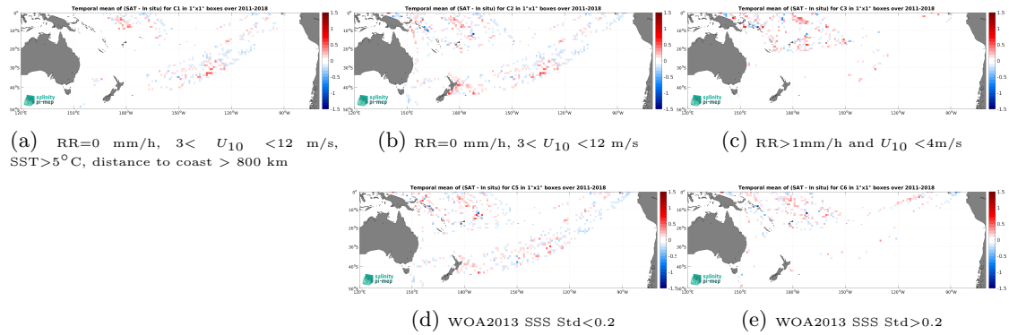
Figure 12: Temporal mean gridded over spatial boxes of size 1^\circ \times 1^\circ of \Delta\text{SSS} (SMOS and SMAP SSS L4 OI v1 - 7 Days (LOPS) - TSG (LEGOS-DM)) for 5 different subdatasets corresponding to:RR=0 mm/h, 3 < U_{10} < 12 m/s, SST >5^\circ\text{C} , distance to coast > 800 km (a), RR=0 mm/h, 3 < U_{10} < 12 m/s (b), RR >1 mm/h and U_{10} < 4 m/s (c), WOA2013 SSS Std <0.2 (d), WOA2013 SSS Std >0.2 (e).
